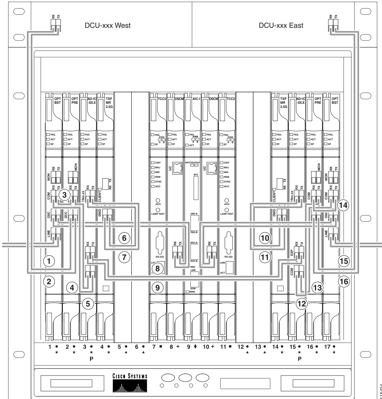
Figure 11-51 Fiberizing an Amplified OADM Node
