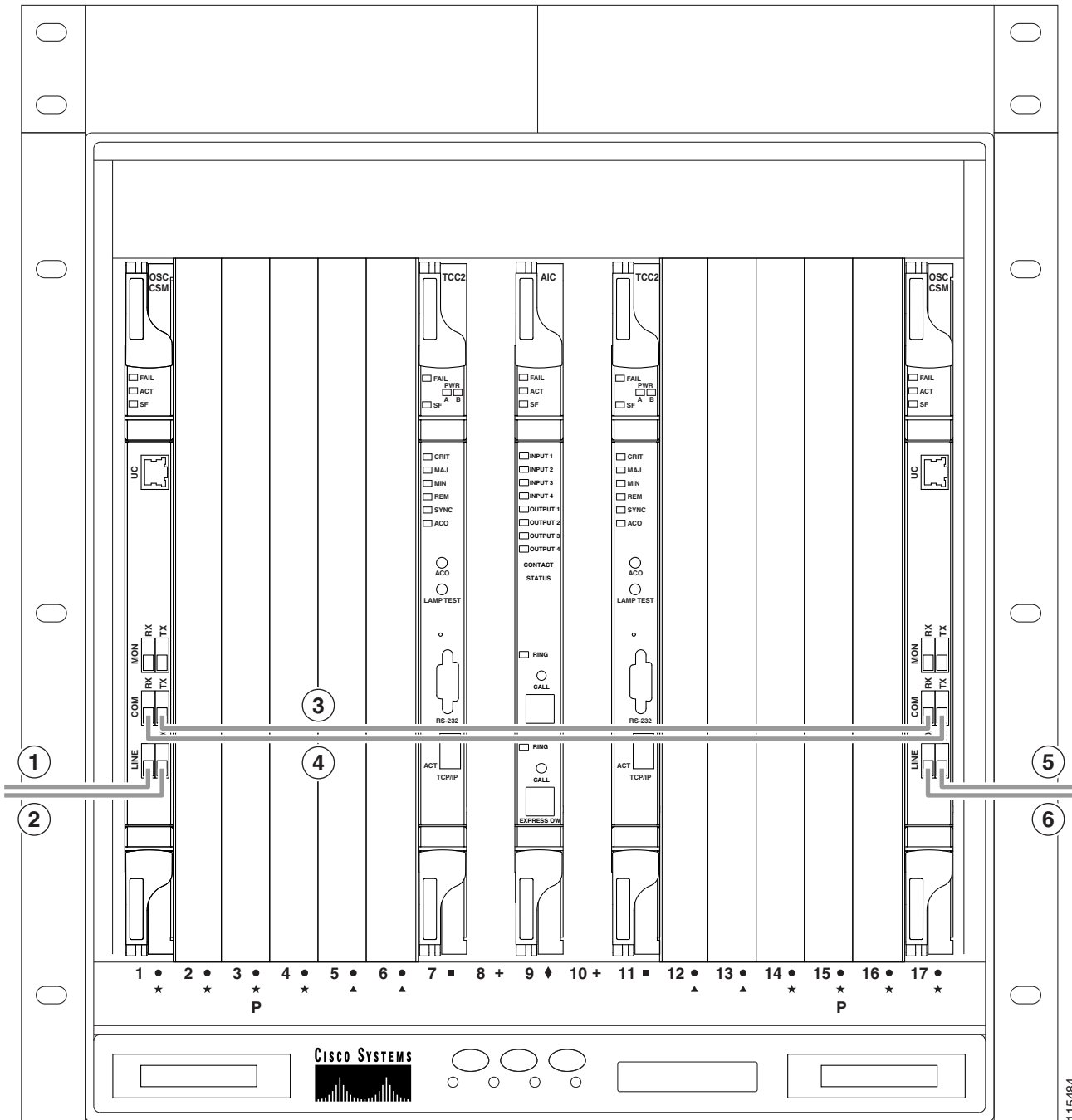
Figure 11-50 Fiberizing an OSC Regeneration Node
