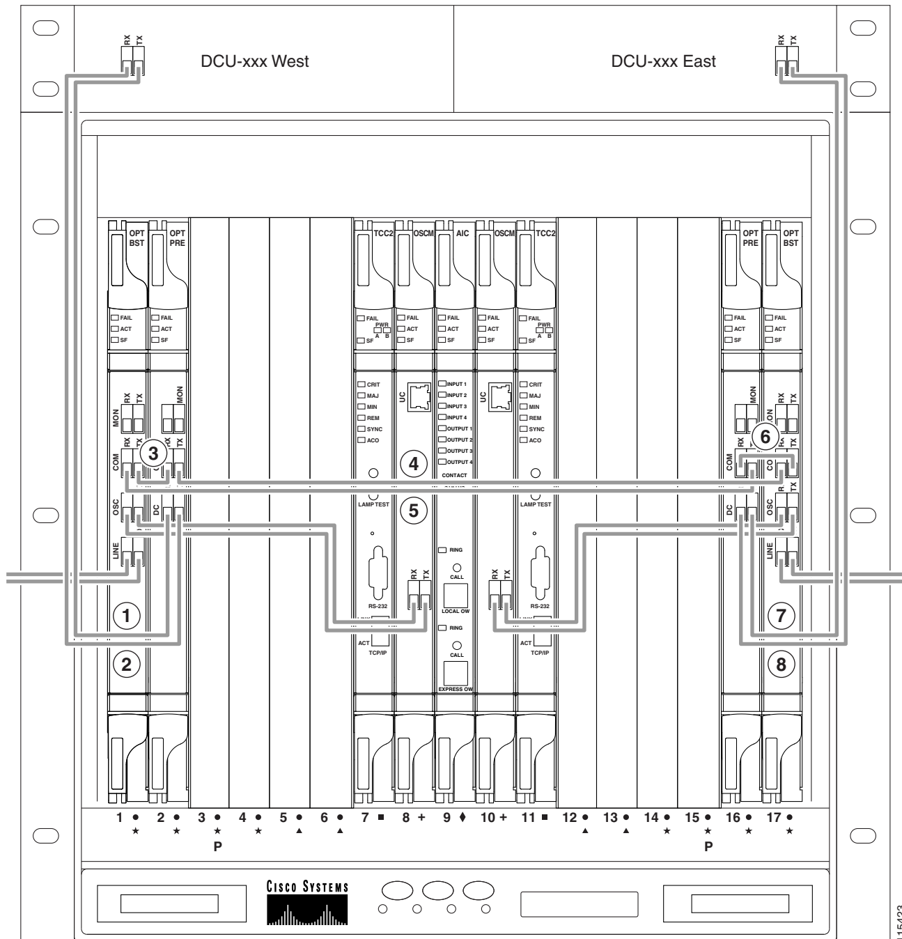
Figure 11-49 Fibering a Line Amplifier Node
