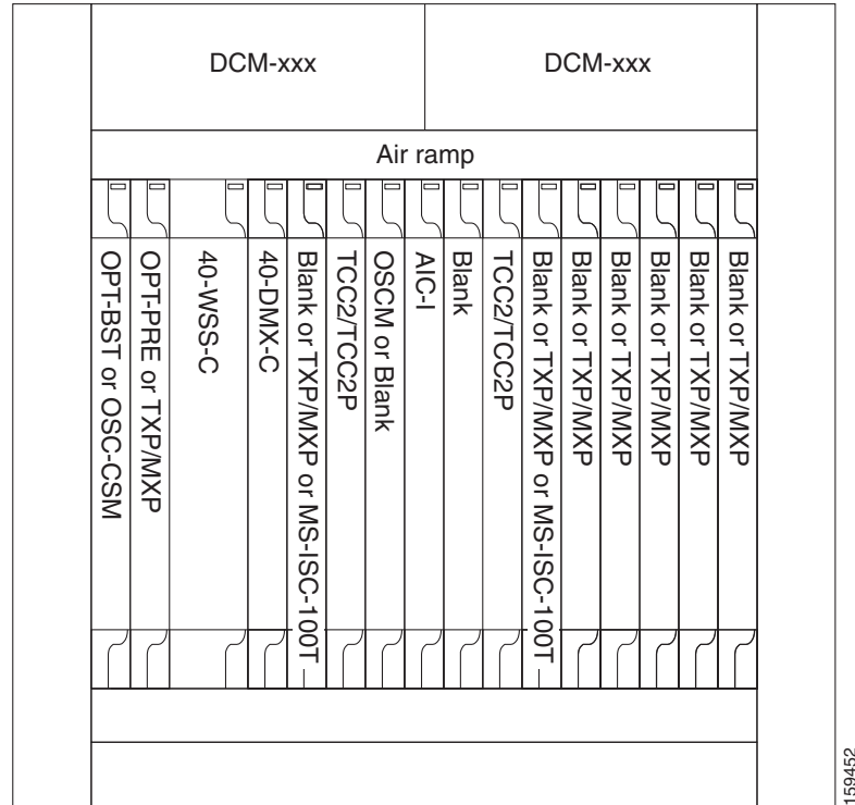
Figure 11-20 Hub Node Configuration Example with 40-WSS-C Cards
