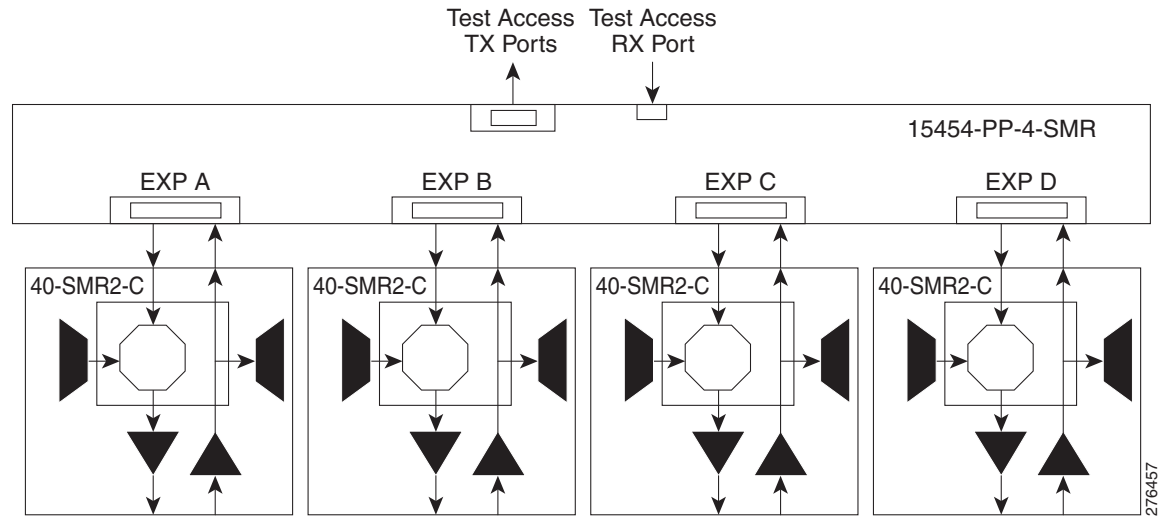
Figure 11-45 15454-PP-4-SMR Patch Panel Signal Flow
