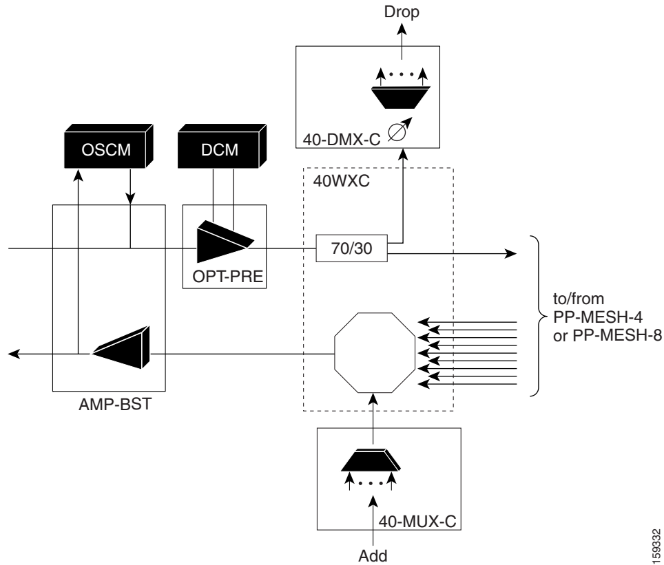
Figure 11-36 Line Termination Mesh Node Side—40-MUX-C Cards
