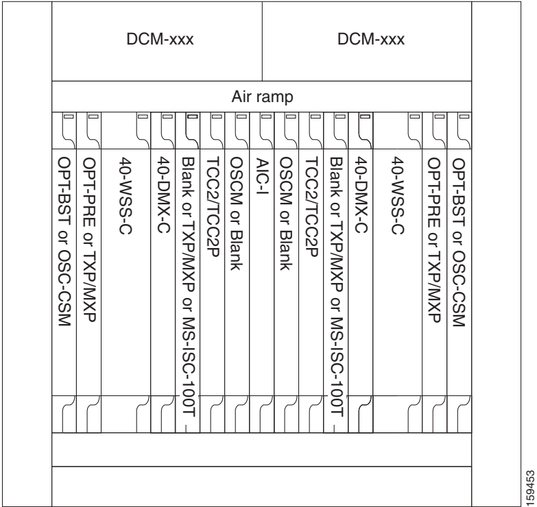
Figure 11-12 ROADM Node with 40-WSS-C Cards Installed
