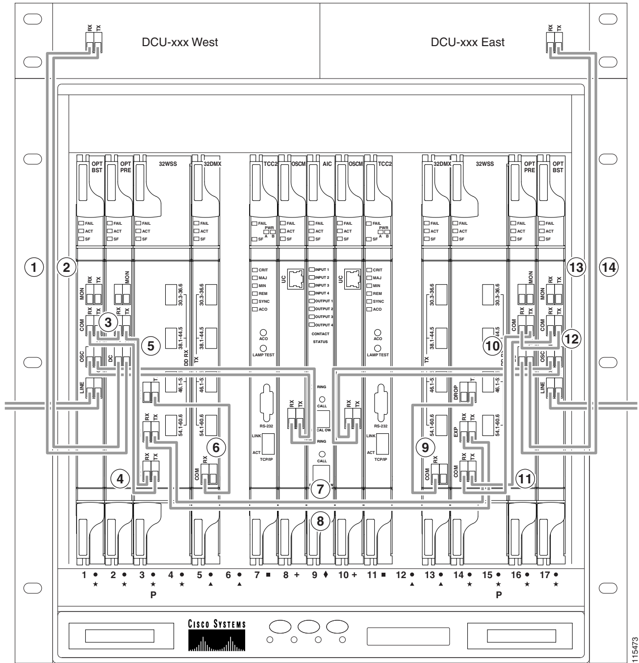
Figure 11-53 Fiberizing a ROADM Node
