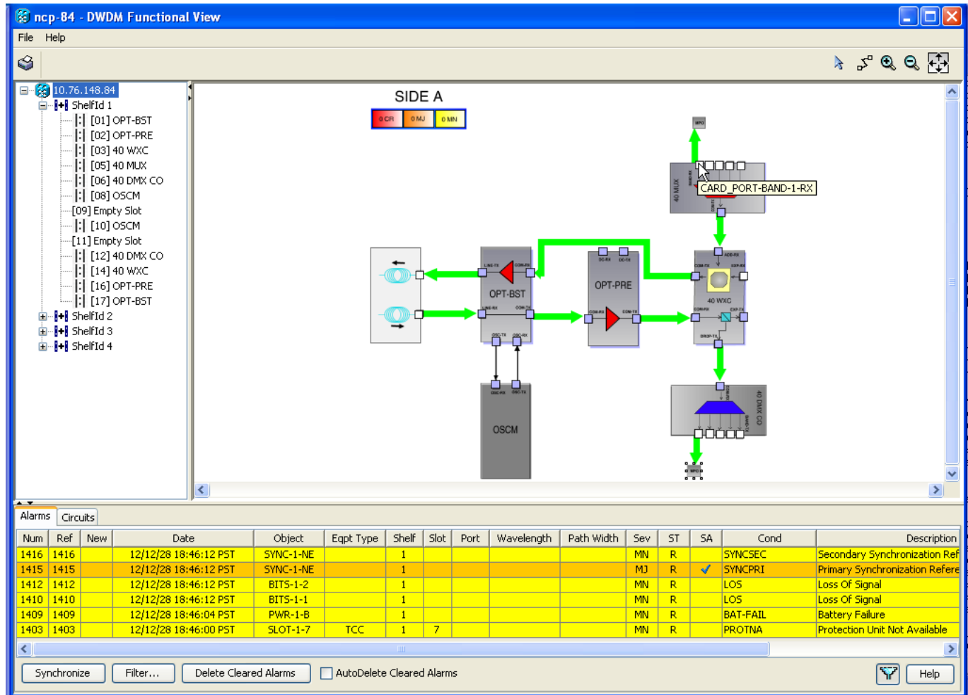
Figure 11-59 Side A 40-MUX Port Information
