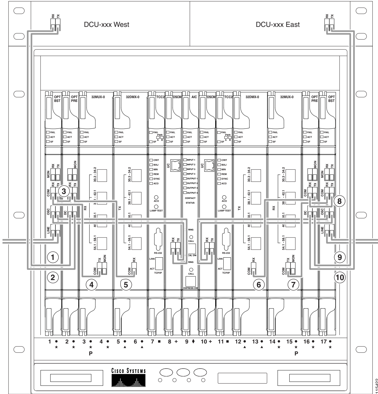
Figure 11-48 Fiberizing a Hub Node
