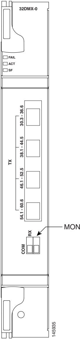
Figure 5-16 32DMX-O Faceplate
