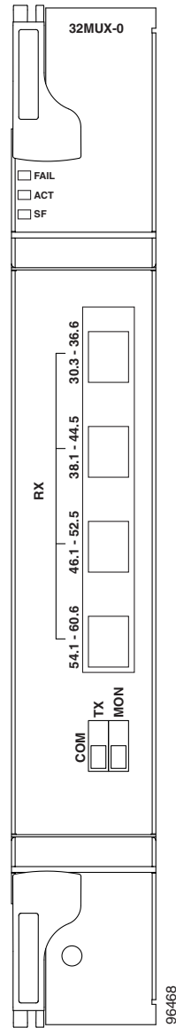
Figure 5-13 32MUX-O Faceplate
