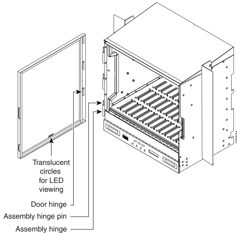
Figure 1-11 Removing the ONS 15454 ANSI Front Door
