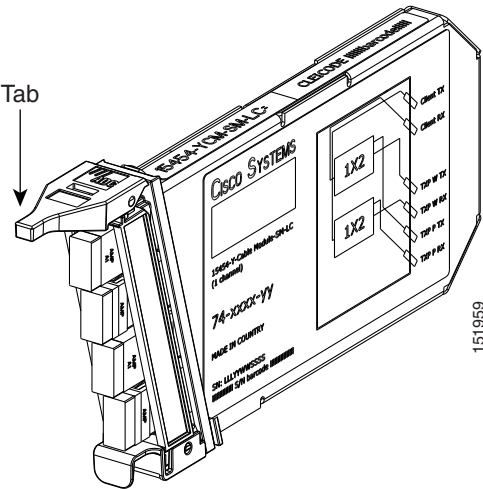
Figure 1-31 Y-Cable Module
