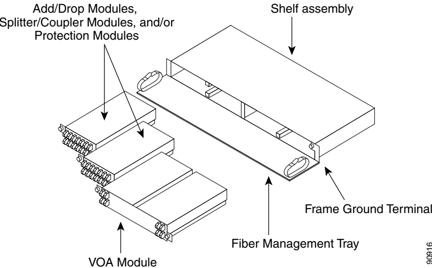
Figure 1-30 ONS 15xxx FlexLayer Shelf Assembly
