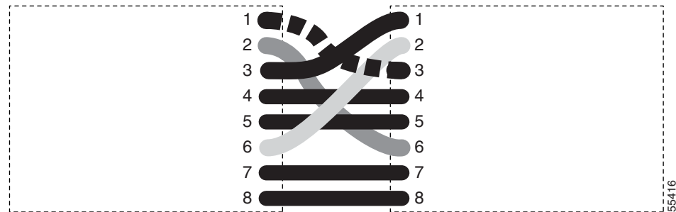
Figure 1-54 Cross-Over Cable Layout
