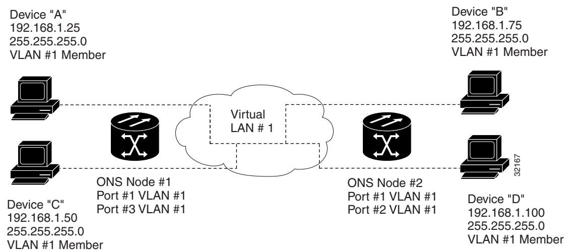
Figure 1-49 Ethernet Connectivity Reference
