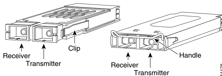
Figure 1-55 GBICs
