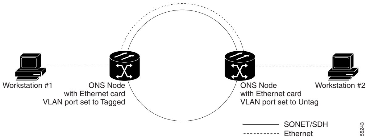
Figure 1-50 VLAN with Ethernet Ports at Tagged and Untag
