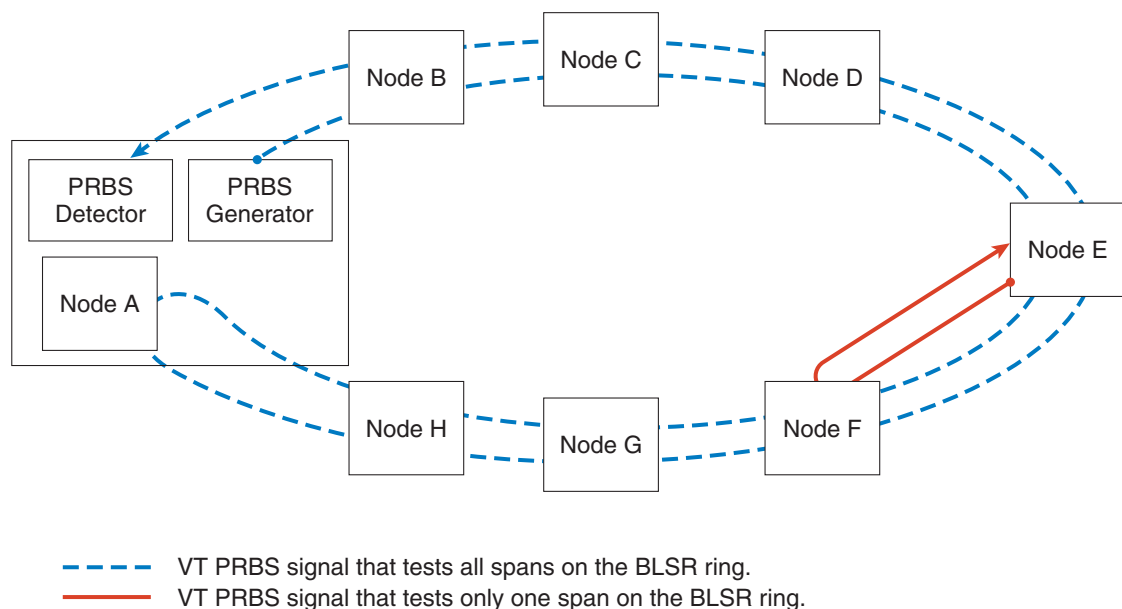
Figure 1-45 CTC Node View Diagnostic Window
