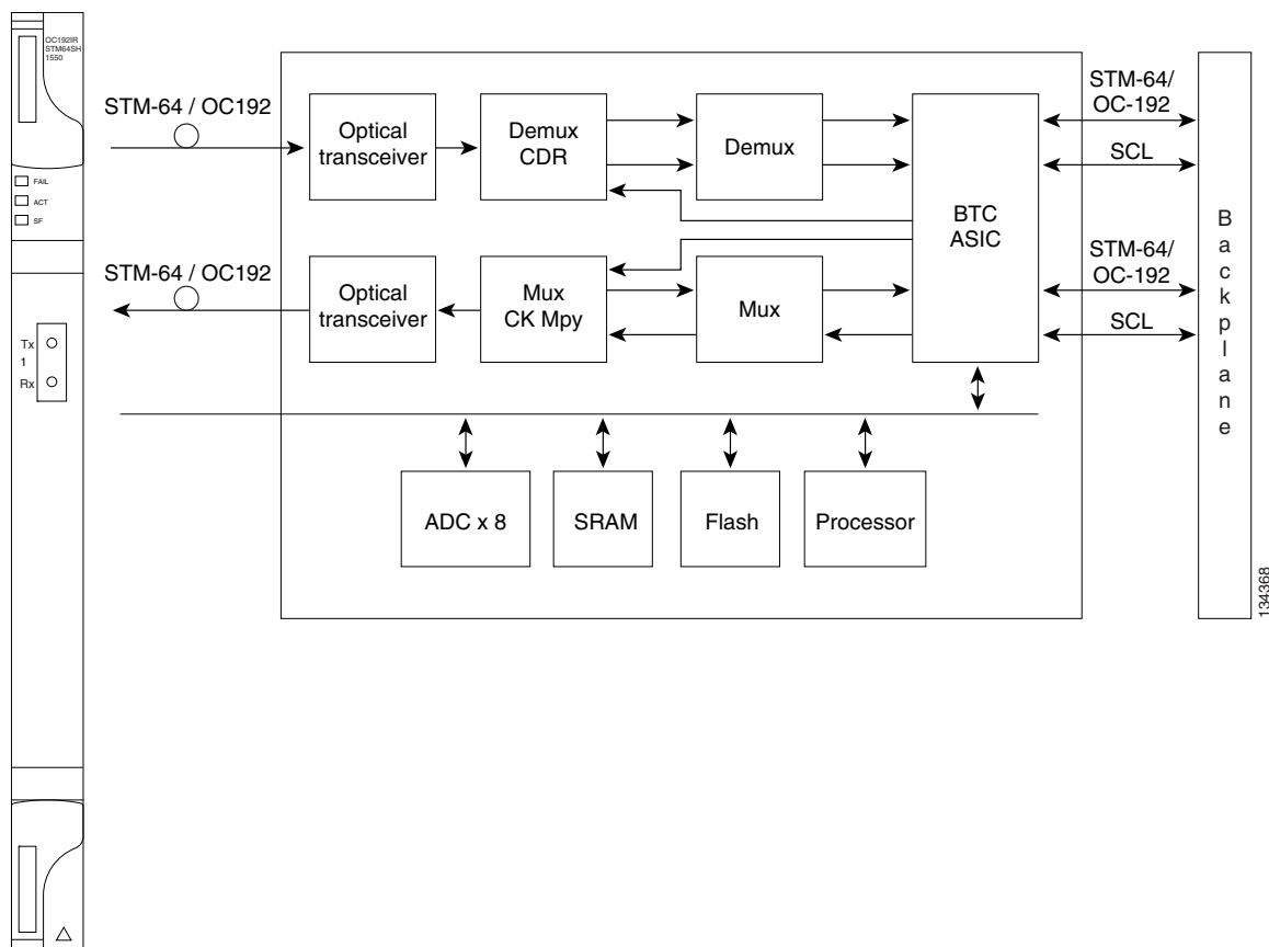
Figure 4-14 OC192 IR/STM64 SH 1550 Faceplate and Block Diagram
