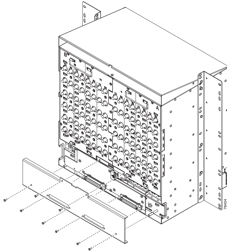
Figure 1-5 Installing the AEP Cover
