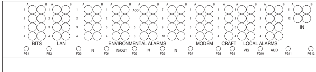
Figure 17-10 Cisco ONS 15454 Backplane Pinouts (Release 3.4 or Later)
