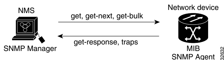
Figure 19-3 Agent Gathering Data from a MIB and Sending Traps to the Manager
