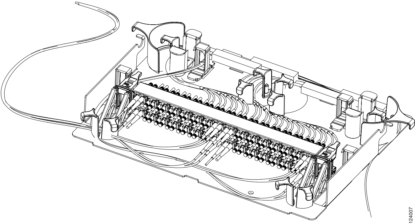
Figure 1-41 Standard Patch-Panel Tray
