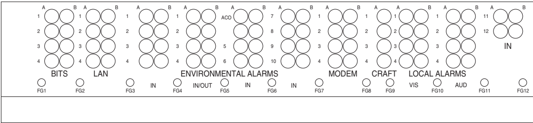
Figure 1-53 Cisco ONS 15454 Backplane Pinouts (Release 3.4 or Later)
