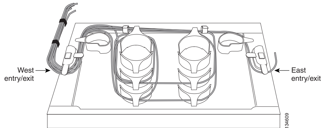
Figure 1-49 Fiber-Storage Tray
