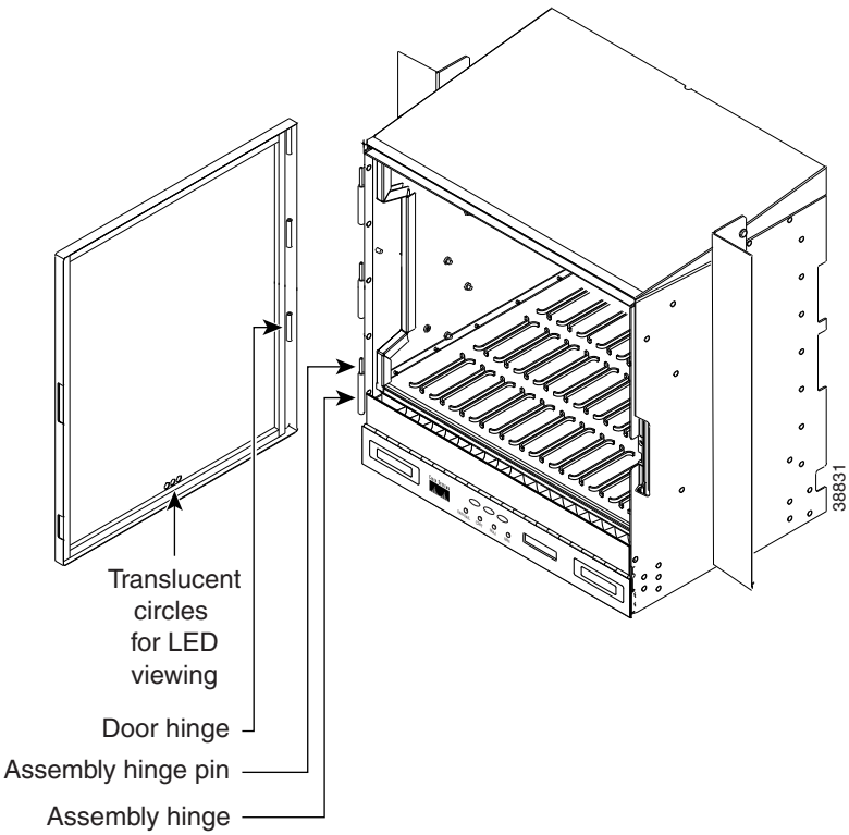
Figure 1-21 Removing the ONS 15454 ANSI Front Door
