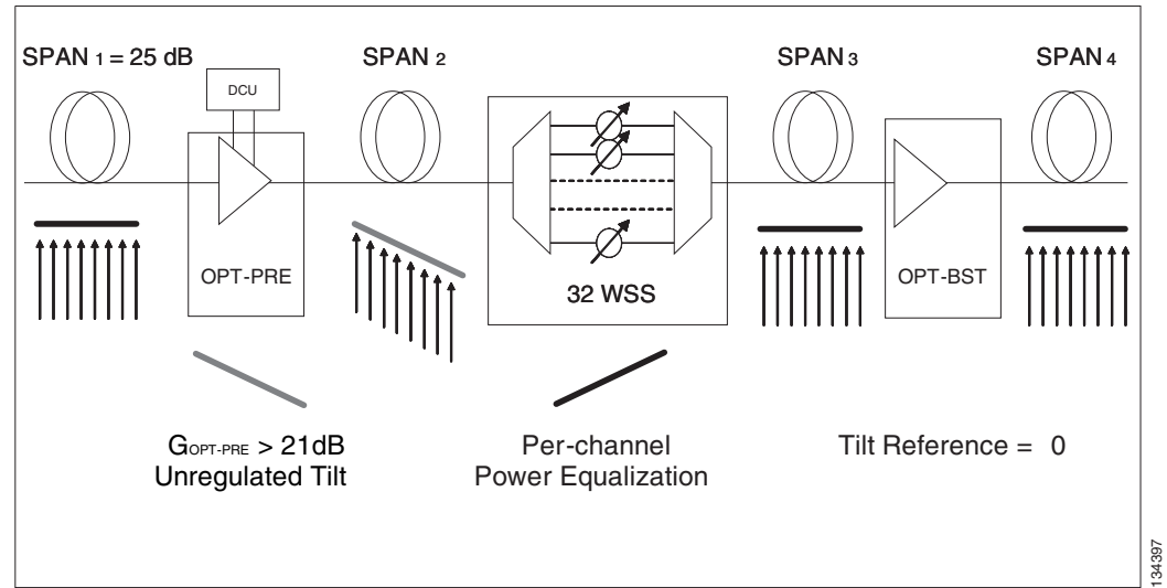
Figure 11-25 System Tilt Compensation With an ROADM Node
