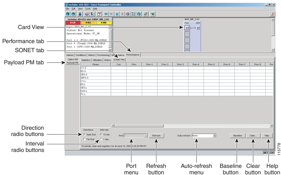
Figure 8-14 SONET PM Tab on the Card View Performance Window
