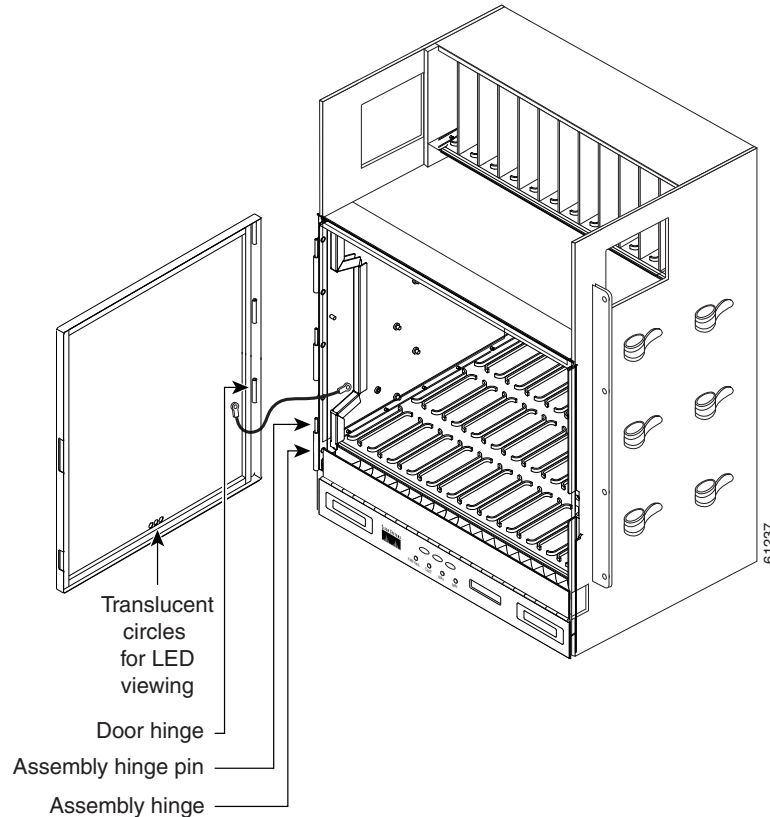
Figure 1-10 Removing the ONS 15454 ETSI Front Door
