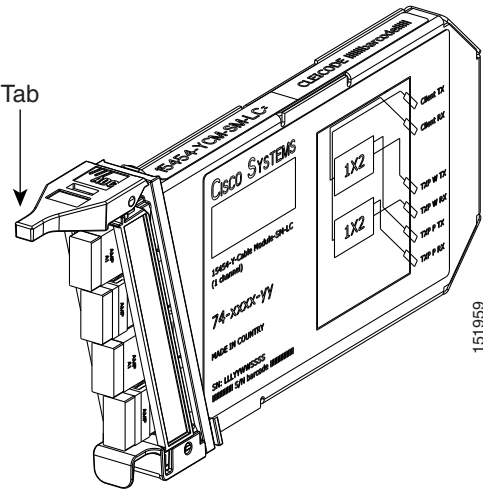
Figure 1-33 Y-Cable Module
