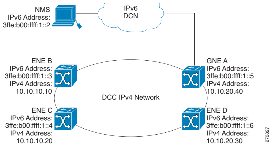
Figure 13-40 IPv6-IPv4 Interaction
