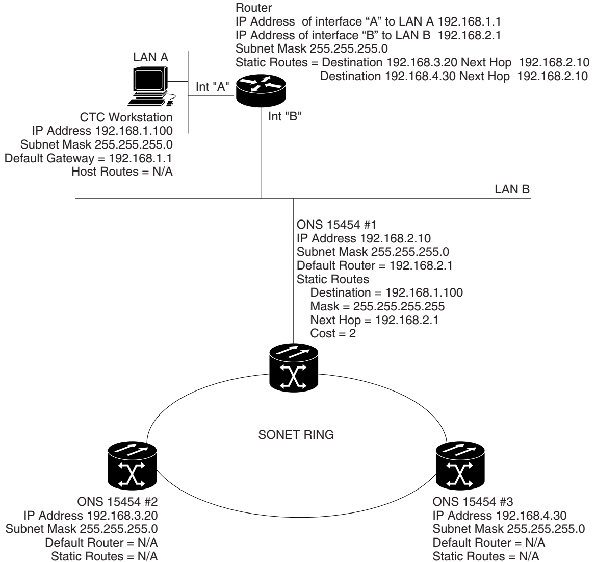
Figure 13-9 IP Scenario 6: OSPF Not Enabled
