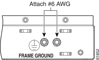
Figure 17-9 Ground Location on the Backplane
