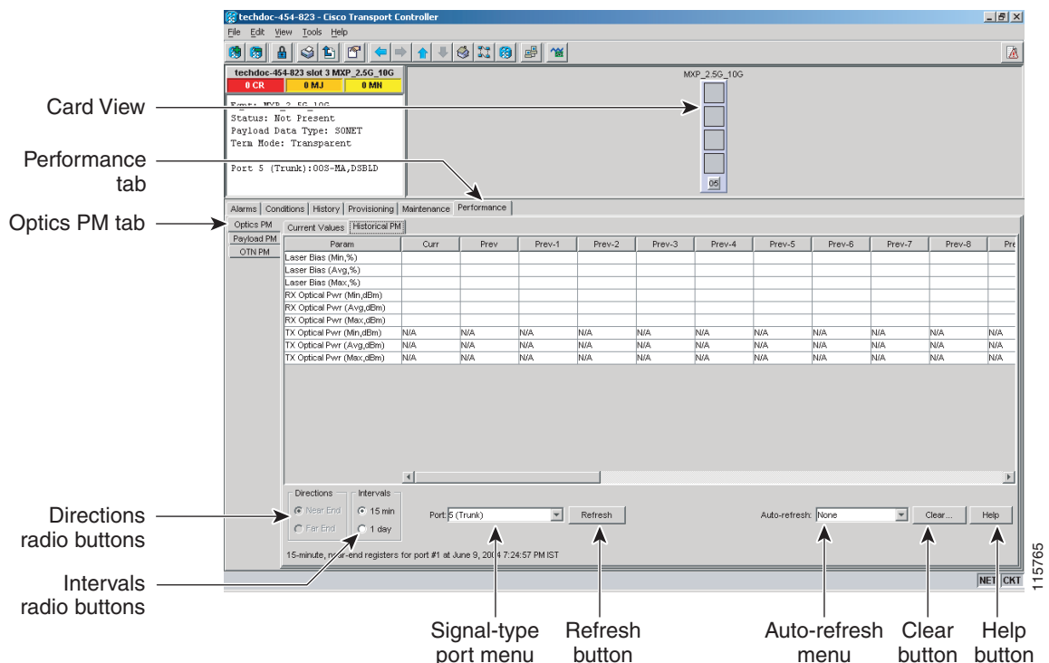
Figure 8-7 Viewing Optics Performance Monitoring Information
