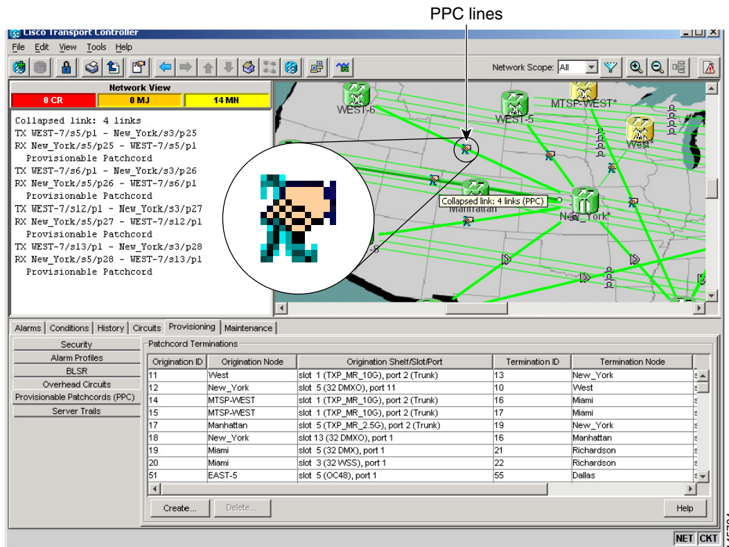
Figure 7-7 Viewing the Provisionable Patchcords Table
