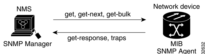
Figure 22-2 SNMP Network
