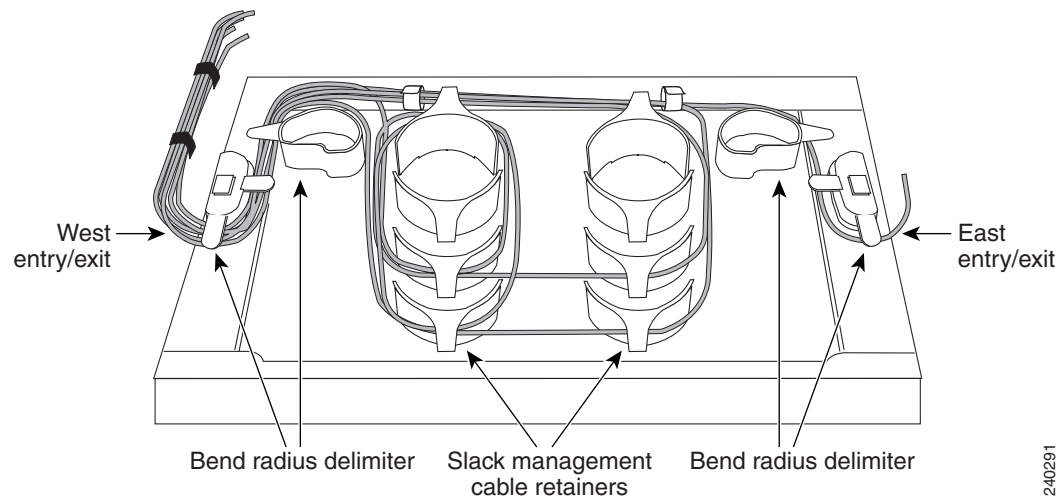
Figure 3-22 Fiber-Storage Tray
