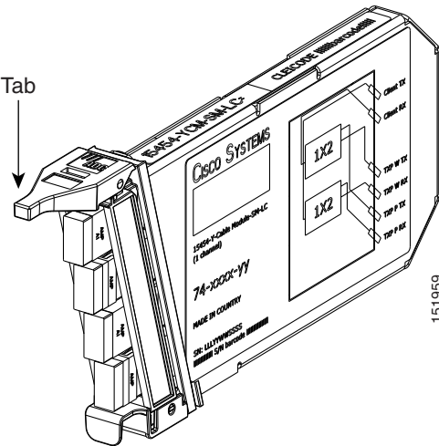
Figure 1-31 Y-Cable Module
