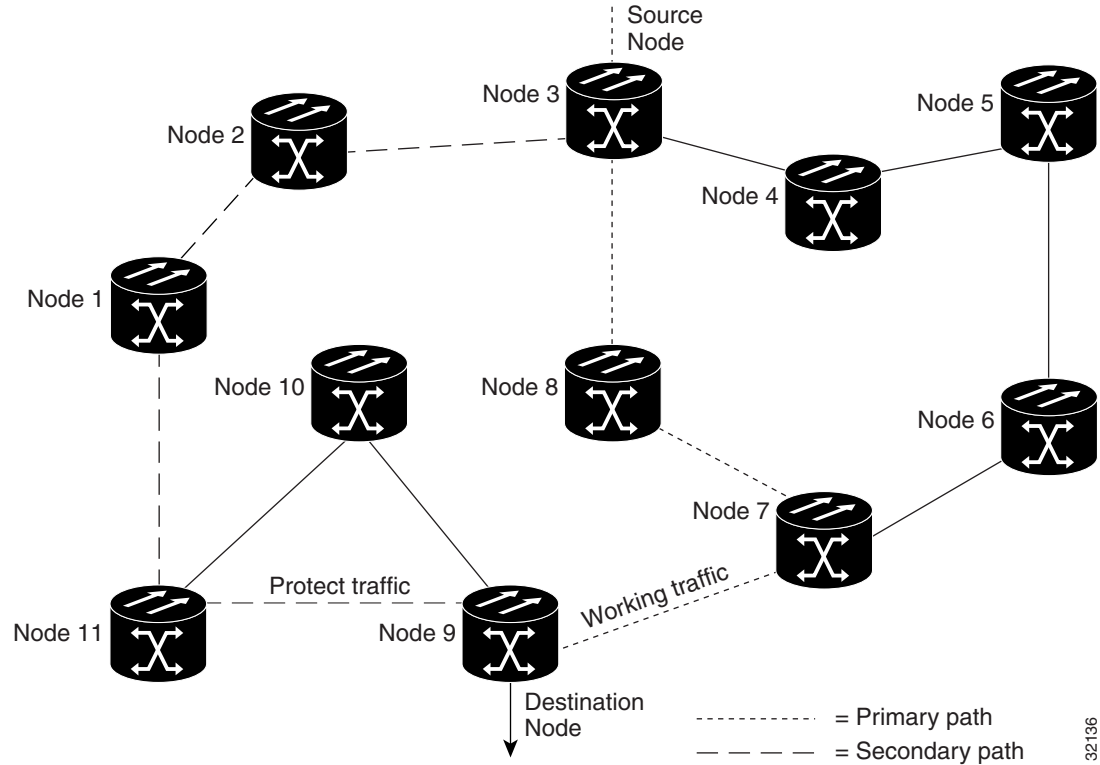
Figure 12-14 Path-Protected Mesh Network
