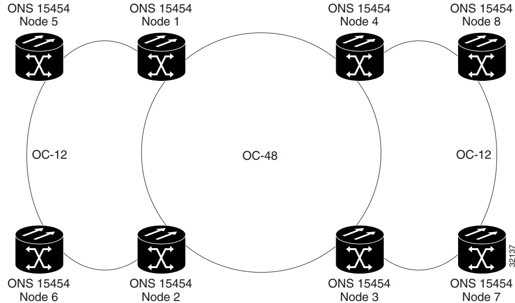
Figure 12-15 PPMN Virtual Ring
