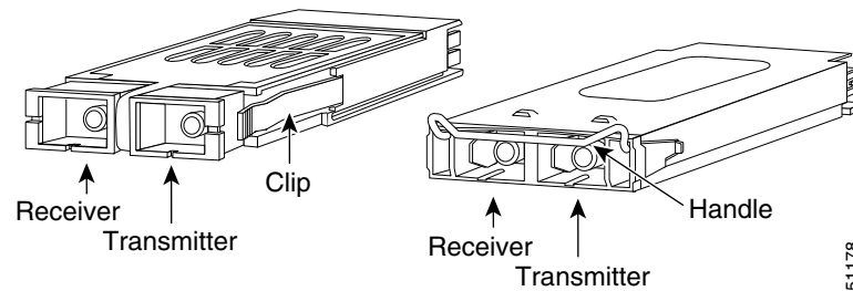
Figure 5-12 GBICs with Clips (left) and with a Handle (right)
