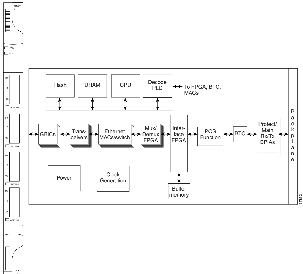
Figure 5-5 G1000-4 Faceplate and Block Diagram
