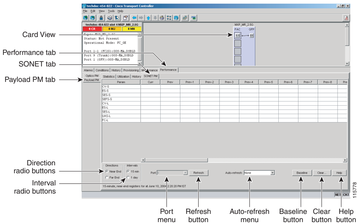
Figure 9-13 SONE PM Tab on the Card View Performance Window
