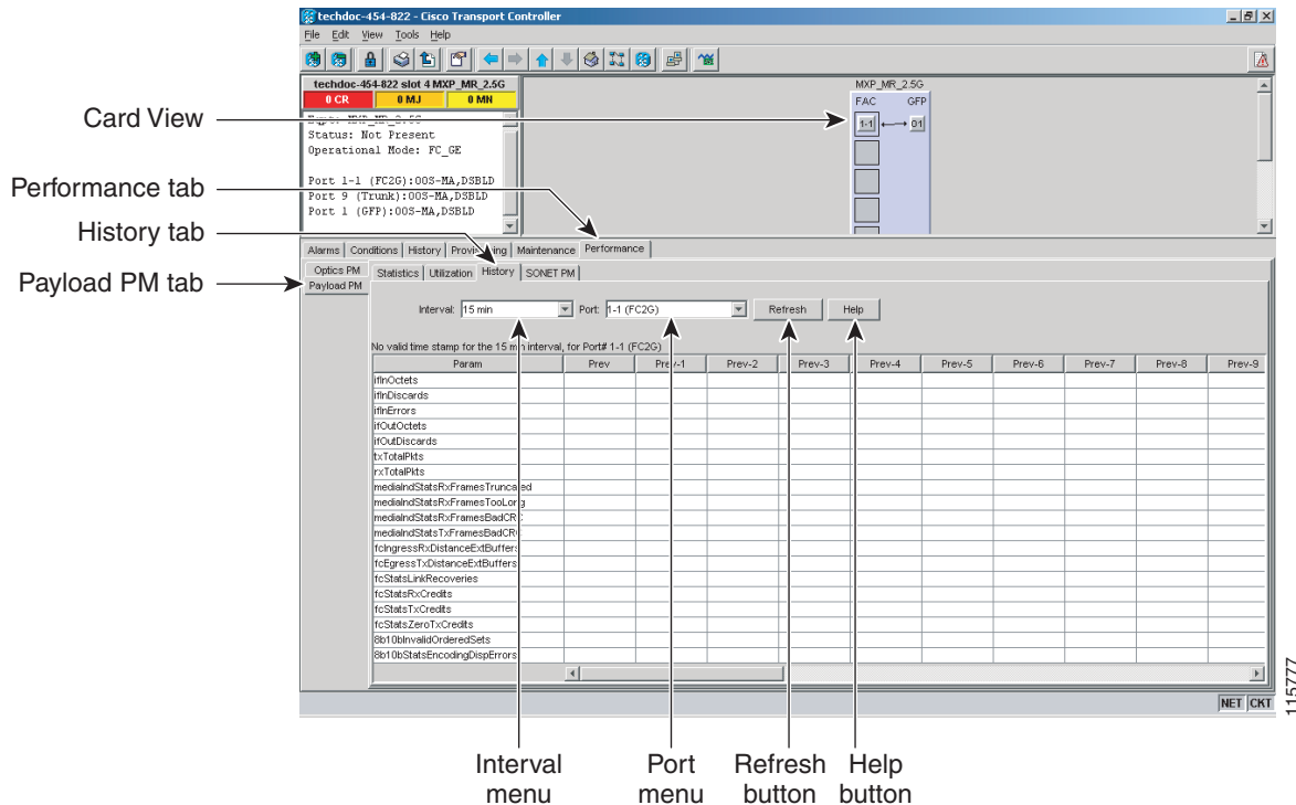
Figure 9-12 History Tab on the Card View Performance Window
