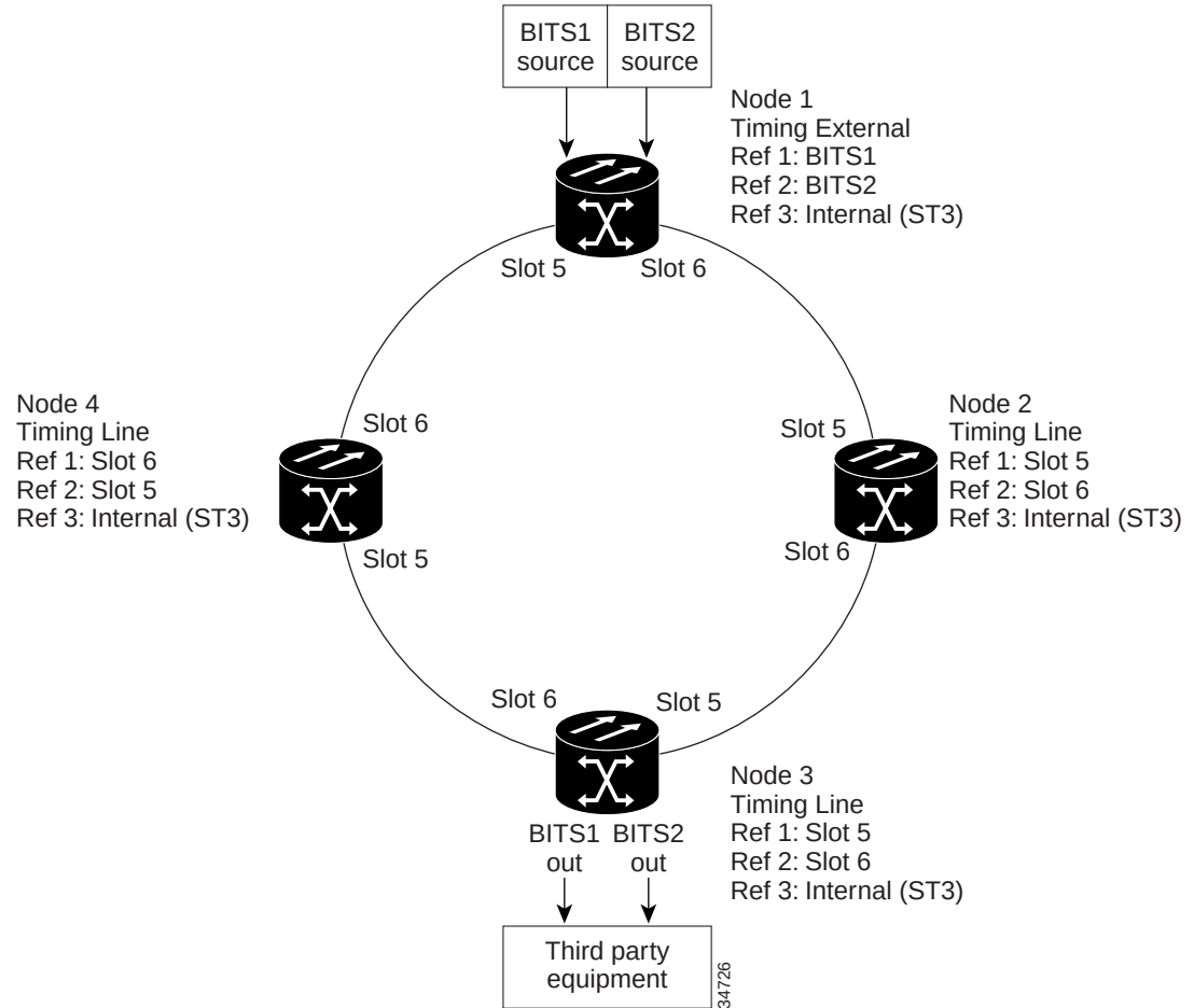
Figure 21-1 ONS 15454 Timing Example
