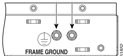
Figure 1-14 Ground Location on the Backplane
