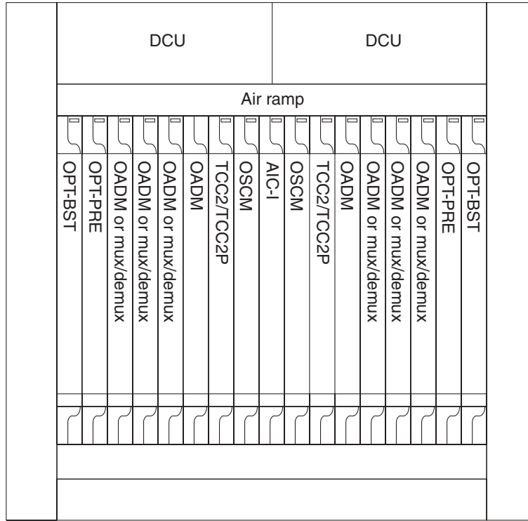
Figure 17-4 Amplified OADM Node Configuration Example
