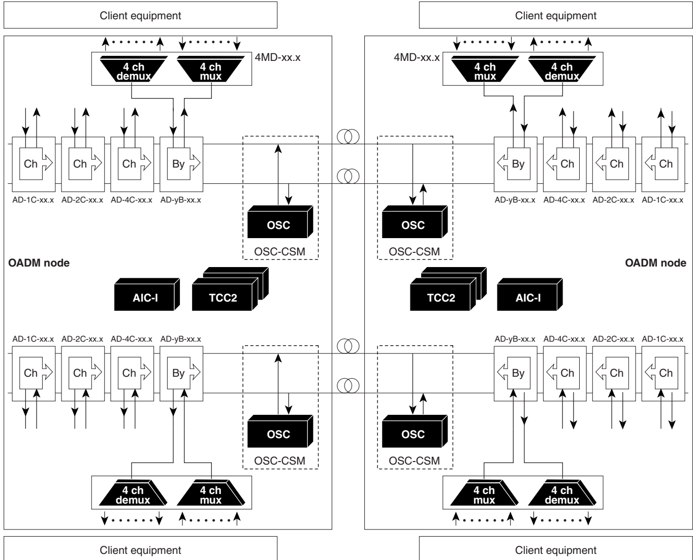
Figure 17-18 1+1 Protected Single-Span Link with Passive OADM Nodes
