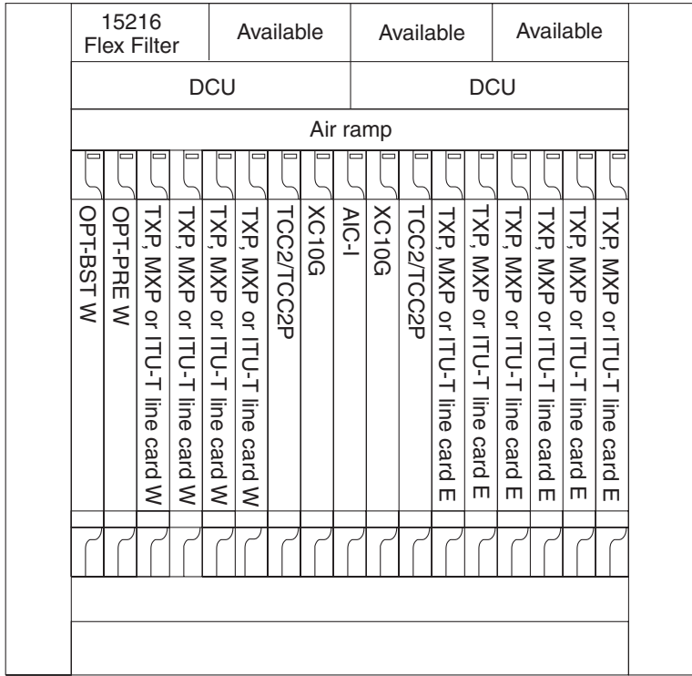
Figure 17-28 Amplified TDM Example with FlexLayer Filters
