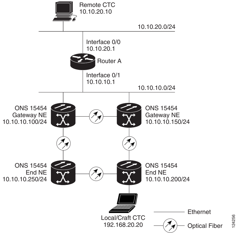
Figure 22-13 Scenario 8: Dual GNEs on the Same Subnet (ANSI and ETSI)
