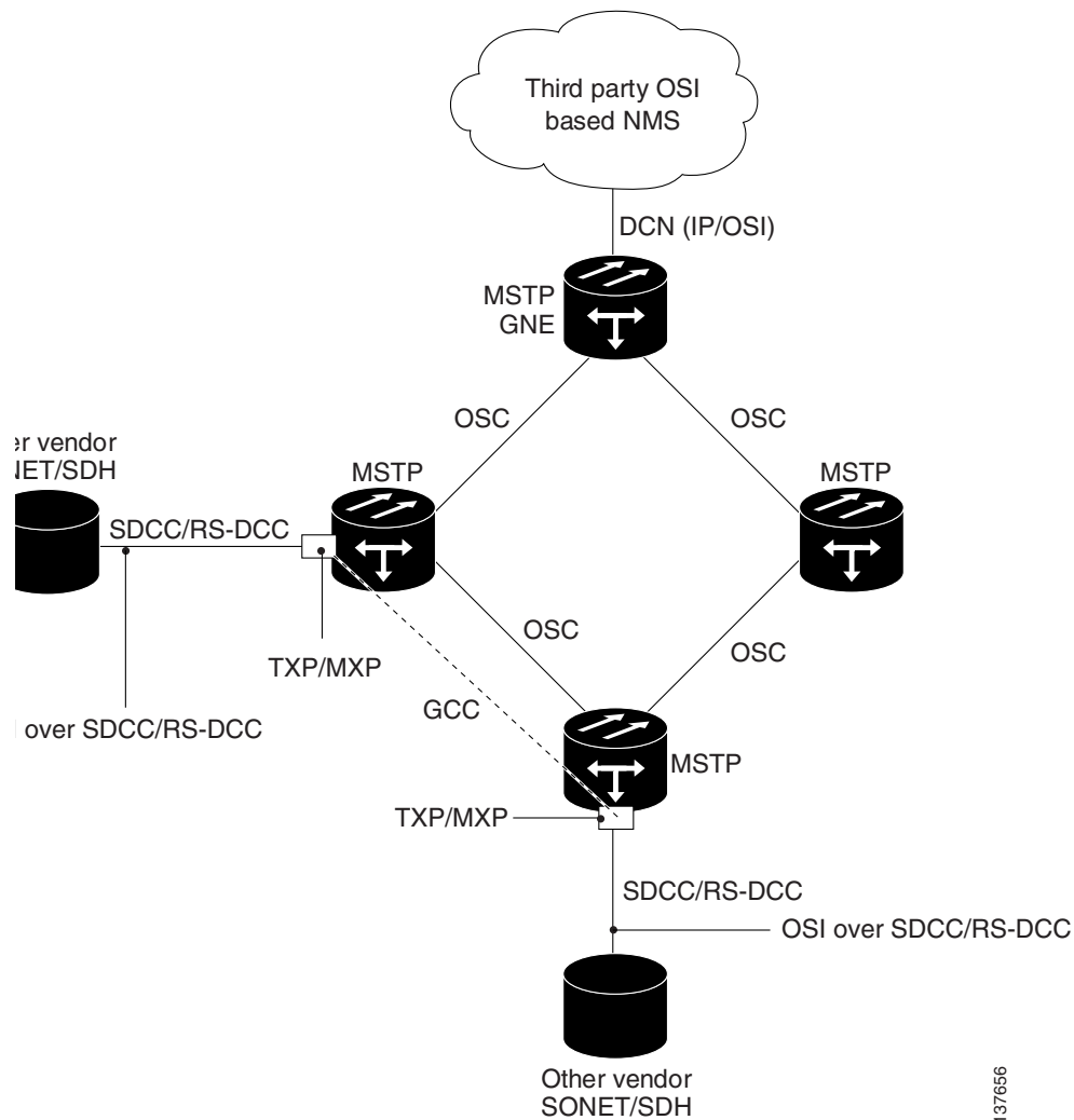
Figure 22-19 OSI/MSTP Scenario 1
