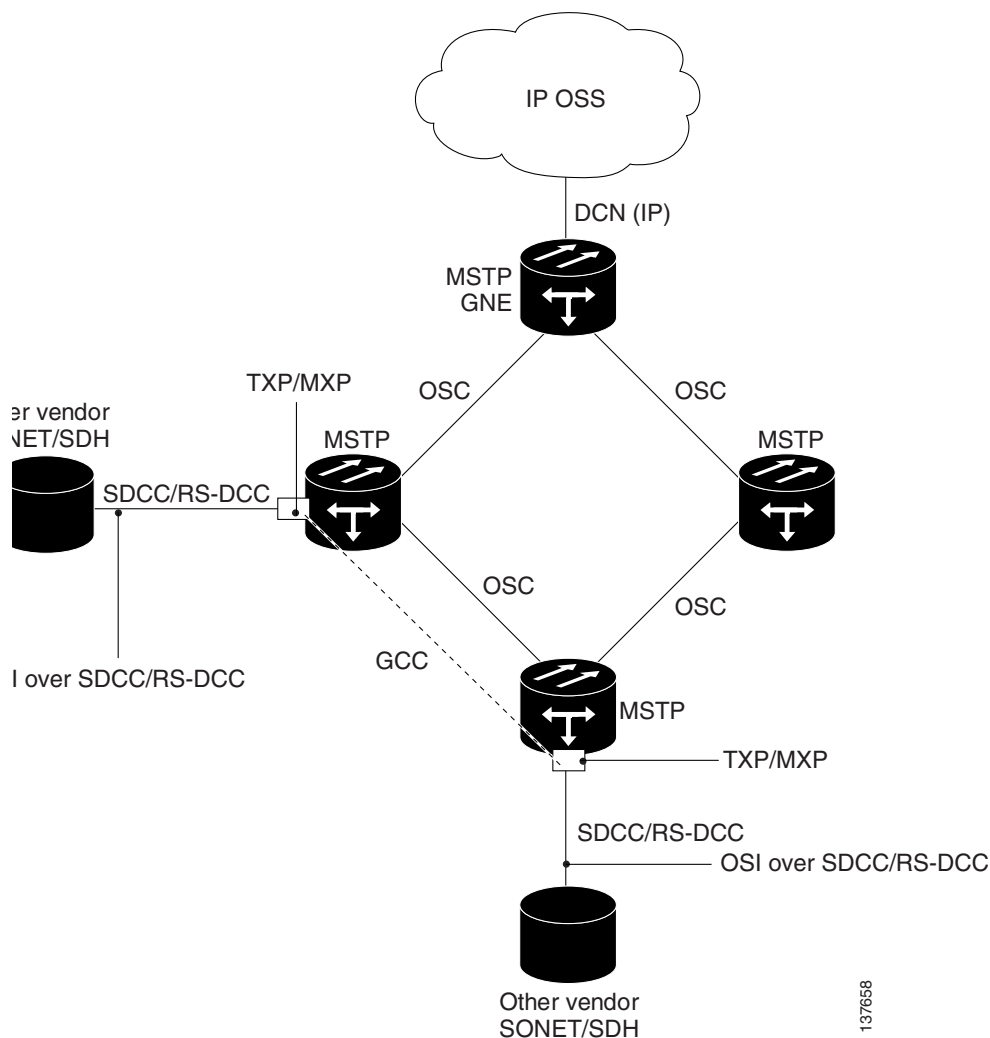
Figure 22-21 OSI/MSTP Scenario 3
