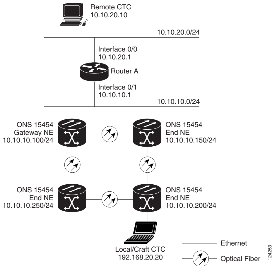
Figure 22-10 Scenario 7: ONS 15454 Proxy Server with GNE and ENEs on the Same Subnet (ANSI and ETSI)
