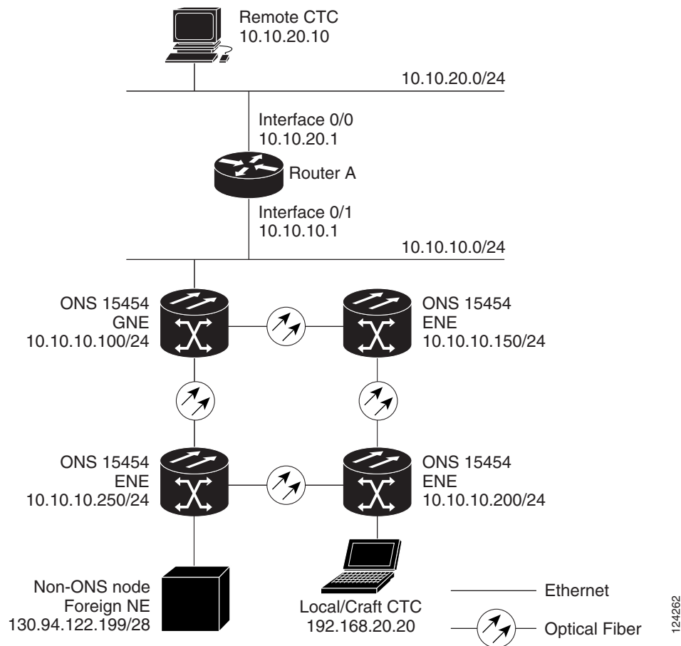
Figure 22-18 Foreign Node Connection to an ENE Ethernet Port
