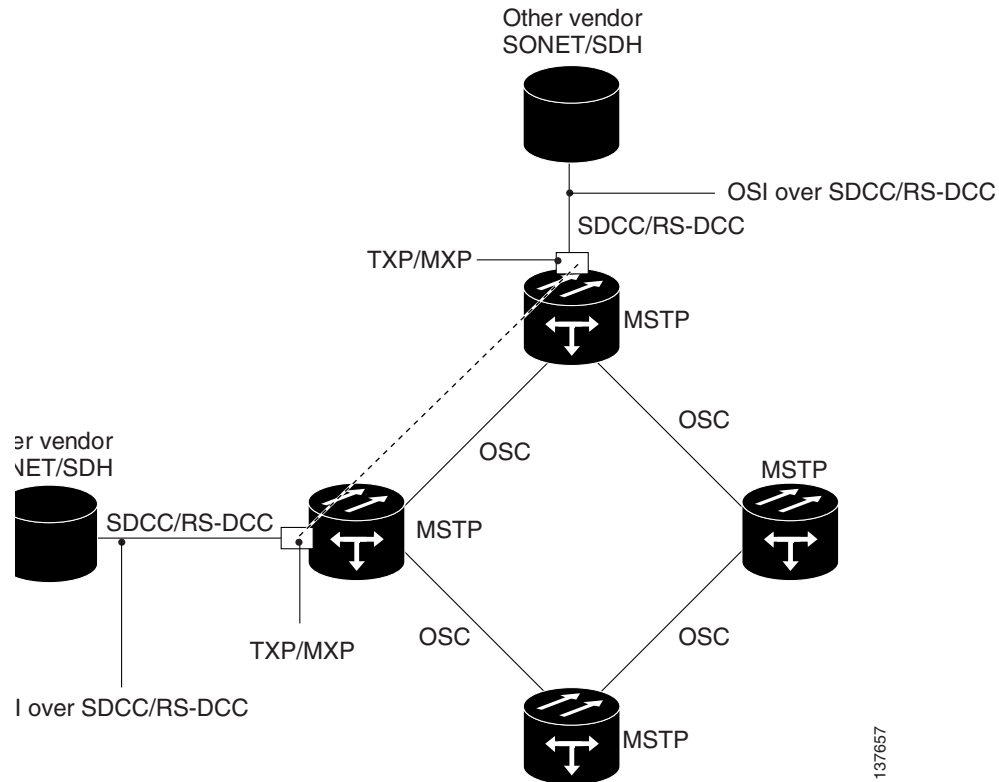
Figure 22-20 OSI/MSTP Scenario 2
