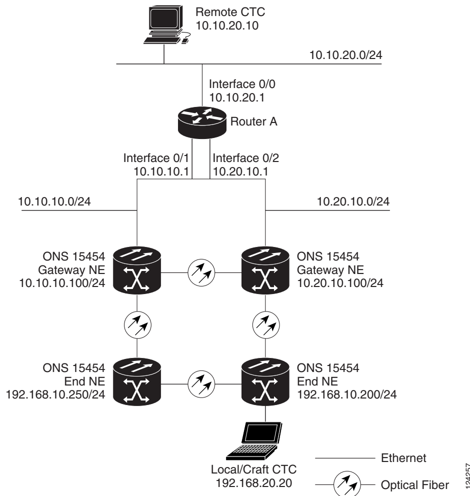
Figure 22-14 Scenario 8: Dual GNEs on Different Subnets (ANSI and ETSI)
