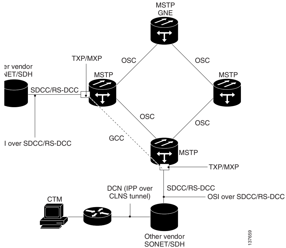
Figure 22-22 OSI/IP Scenario 4
