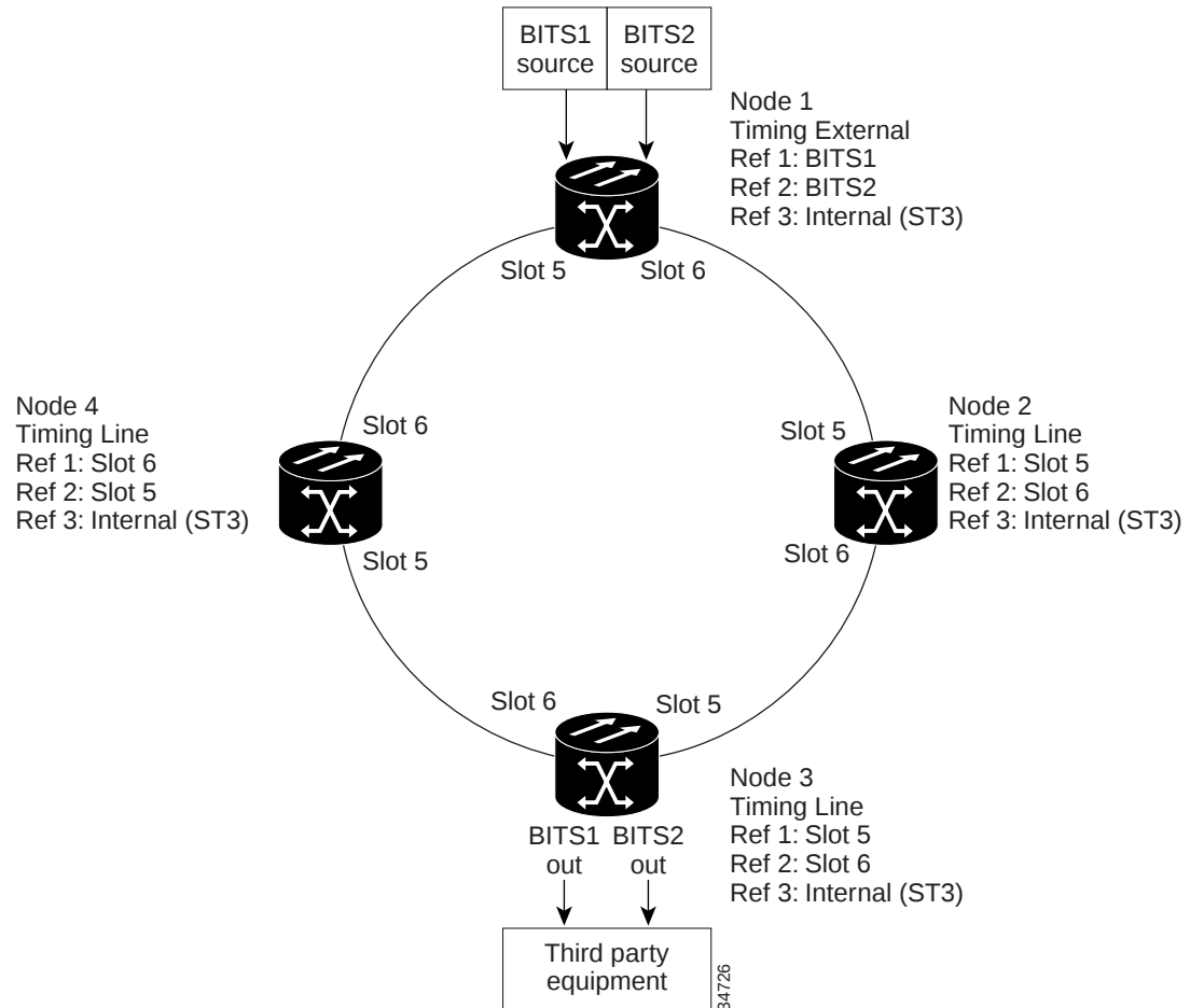
Figure 19-1 ONS 15454 Timing Example
