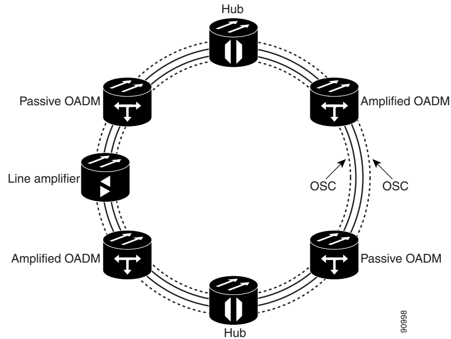
Figure 17-2 Multihubbed Ring
