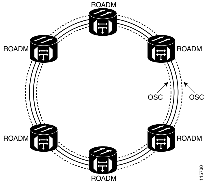
Figure 17-3 Any-to-Any Ring
