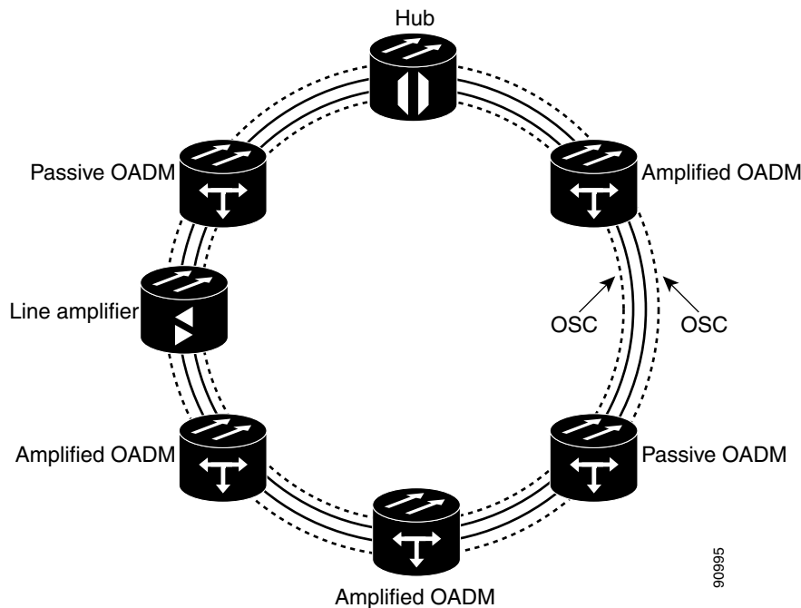
Figure 17-1 Hubbed Ring
