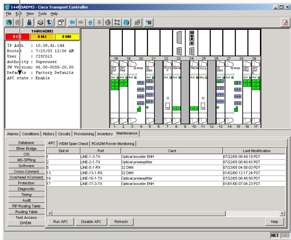
Figure 17-8 Automatic Power Control
