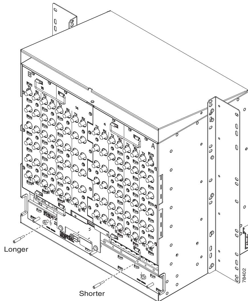
Figure 1-2 Replace Backplane Screws with Standoffs
