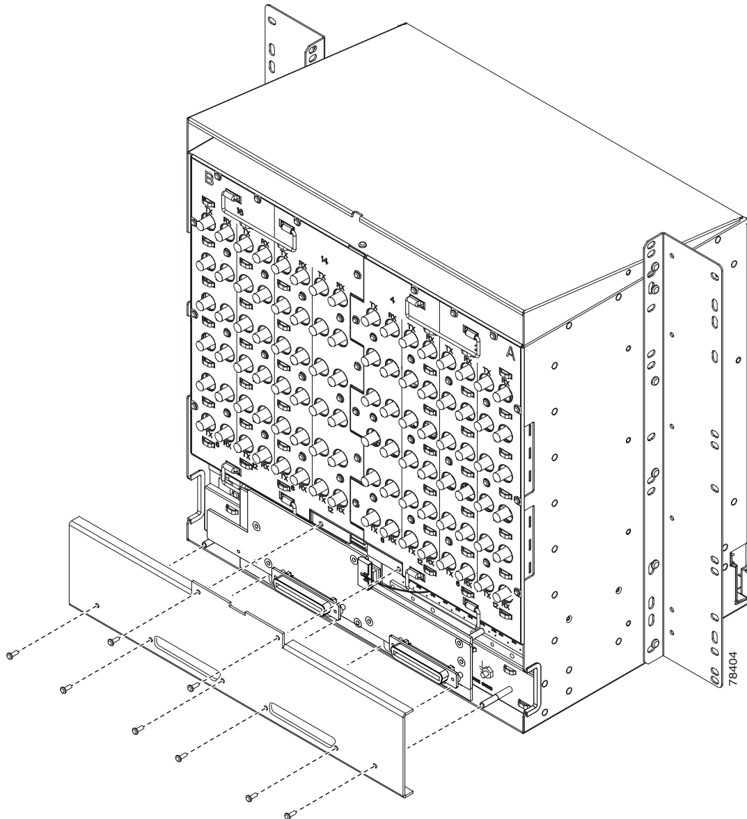
Figure 1-5 Installing the AEP Cover
