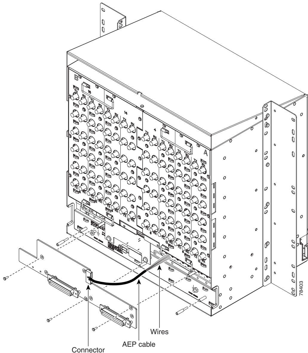
Figure 1-3 Installing Standoffs and the AEP
