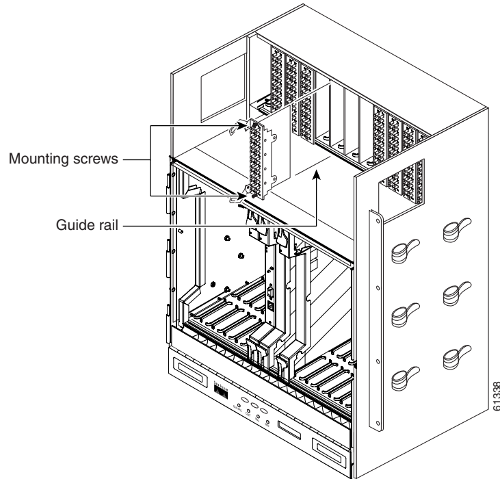
Figure 1-11 Installing FMECs on the ONS 15454 ETSI
