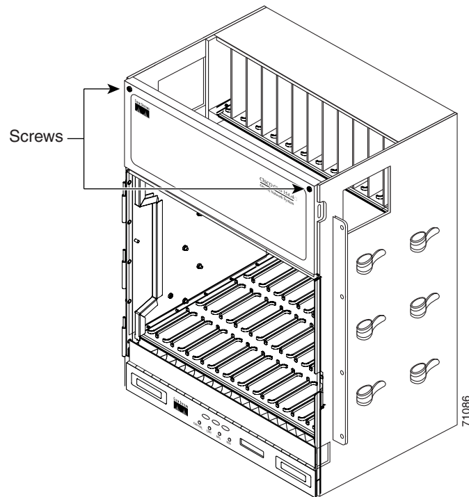
Figure 1-9 Unscrewing the FMEC Cover
