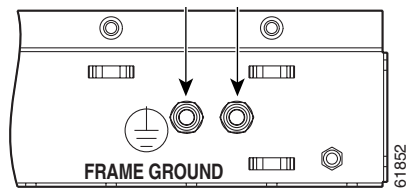
Figure 1-13 Ground Location on the Backplane
