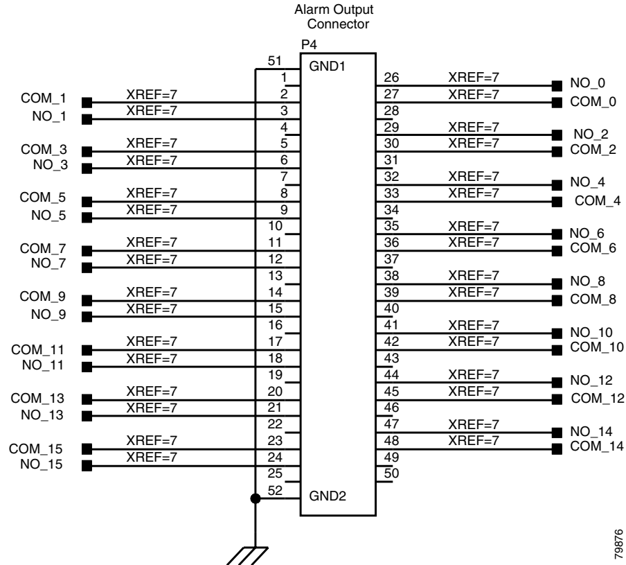
Figure 1-24 Alarm Output Connector
