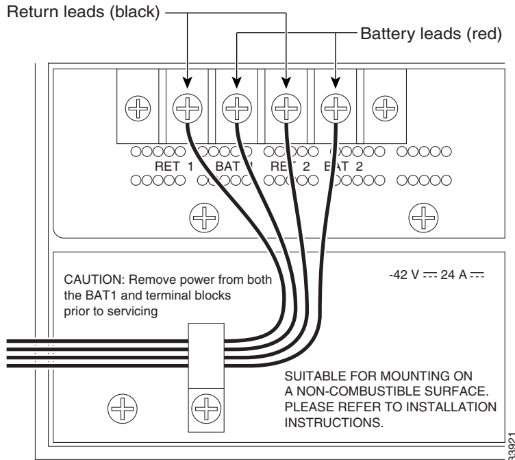
Figure 1-14 Cisco ONS 15454 Power Terminals
