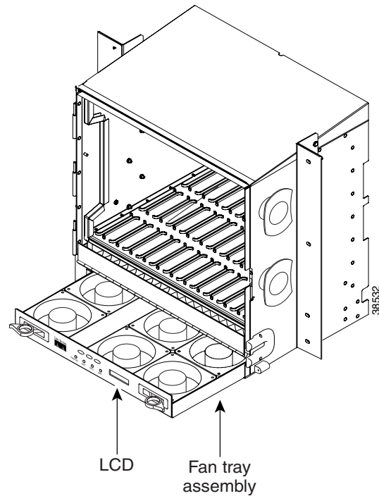
Figure 1-16 Installing the Fan-Tray Assembly on the ONS 15454 ANSI
