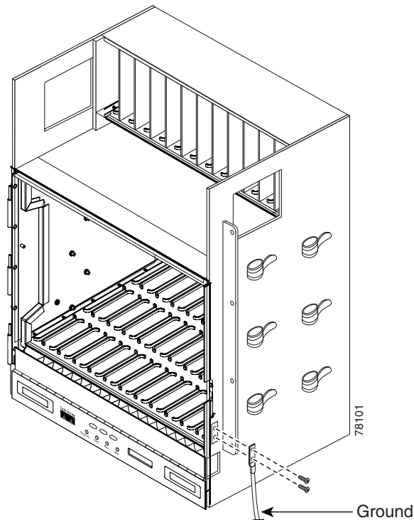
Figure 1-12 Grounding the ONS 15454 ETSI
