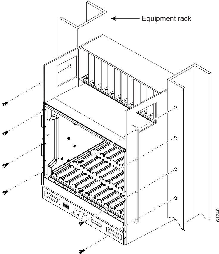
Figure 1-3 Mounting an ONS 15454 ETSI in a Rack
