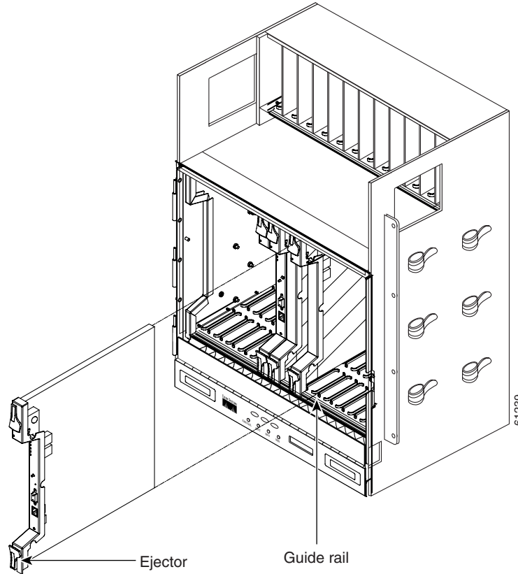
Figure 1-29 Installing Cards in the ONS 15454 ETSI
