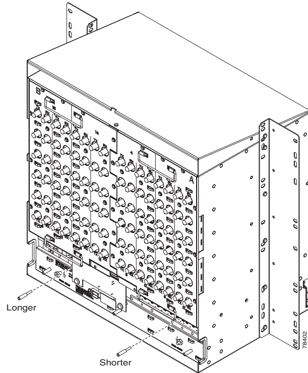
Figure 1-17 Replace Backplane Screws with Standoffs
