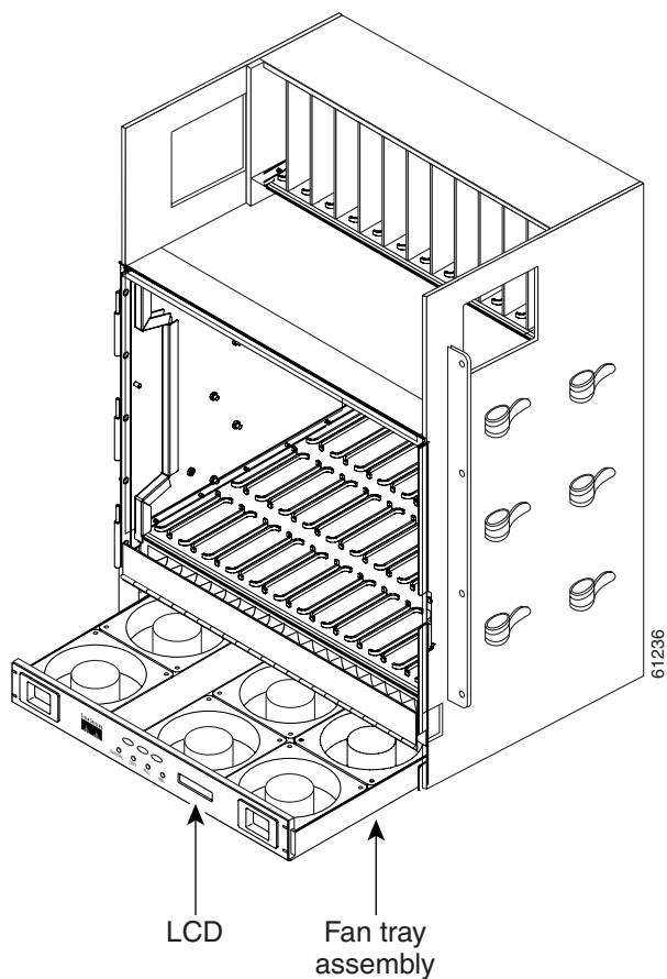
Figure 1-15 Installing the Fan-Tray Assembly on the ONS 15454 ETSI
