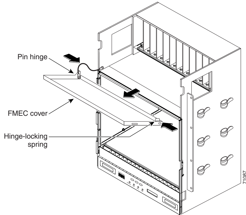
Figure 1-25 ONS 15454 ETSI FMEC Cover
