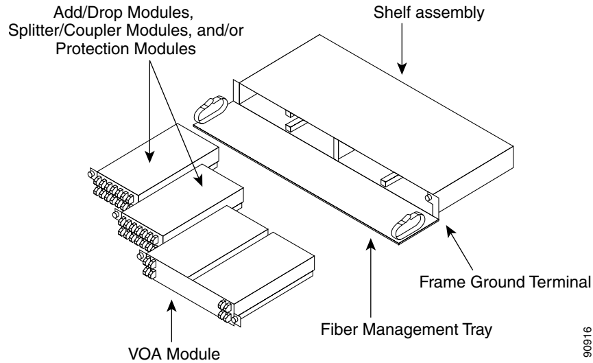
Figure 1-28 ONS 15xxx FlexLayer Shelf Assembly
