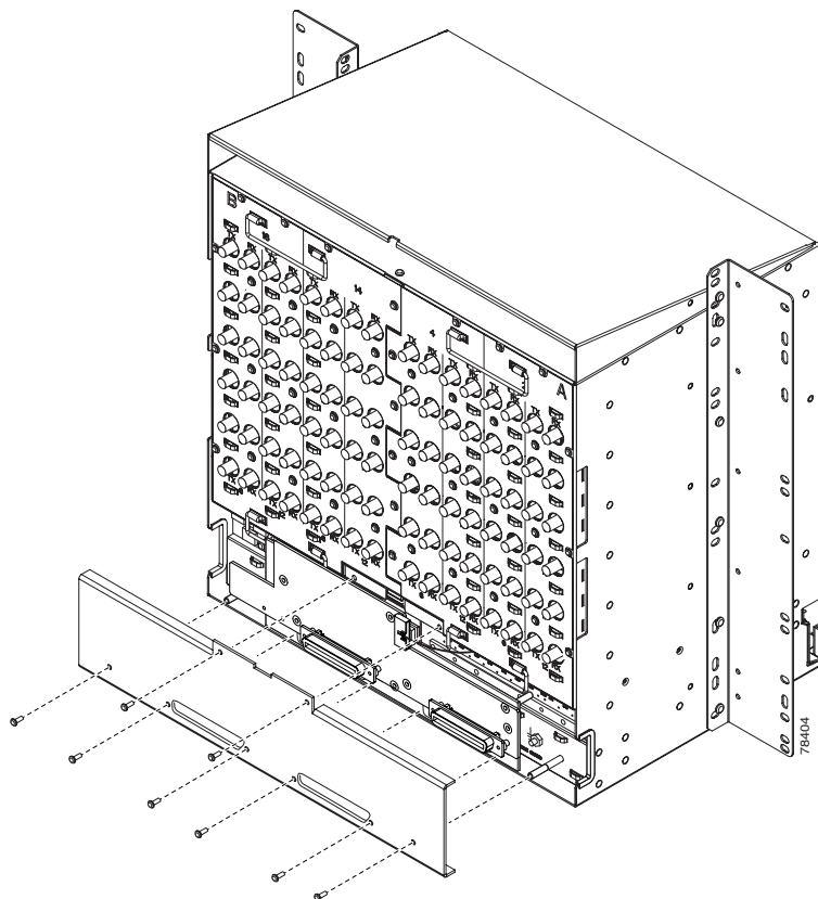
Figure 1-22 Installing the AEP Cover
