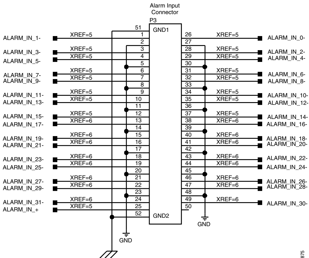
Figure 1-23 Alarm Input Connector
