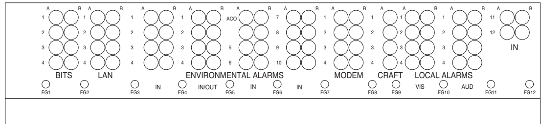
Figure 1-20 Cisco ONS 15454 Backplane Pinouts (Release 3.4 or Later)
