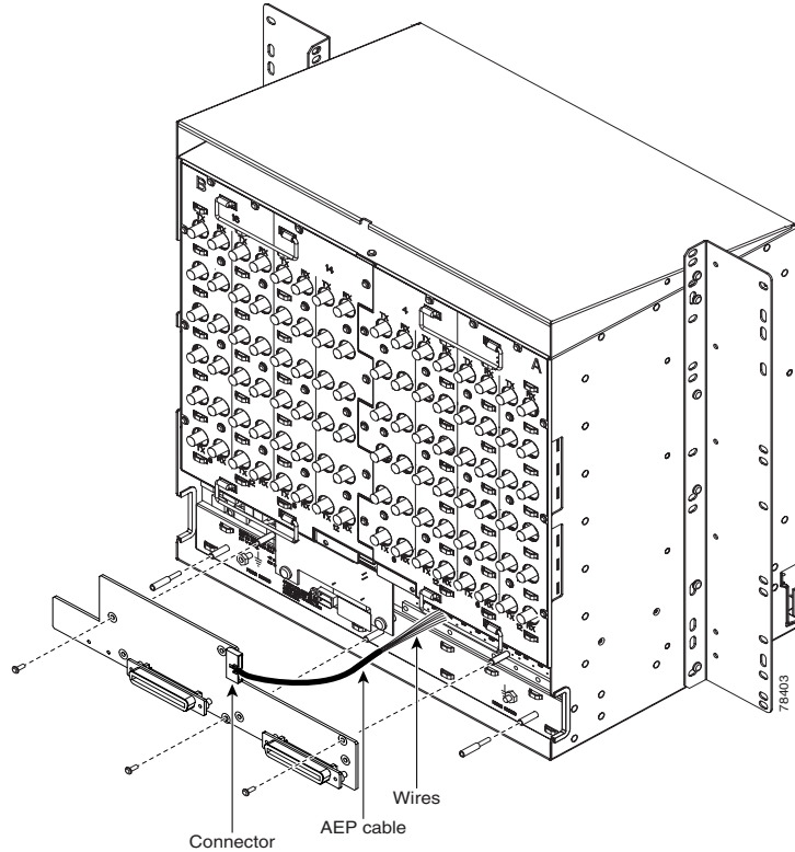
Figure 1-18 Installing Standoffs and the AEP
