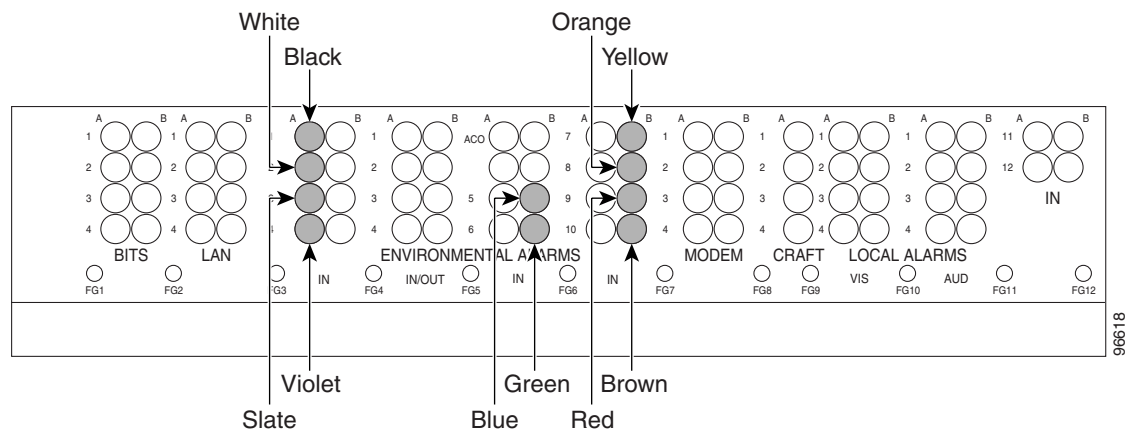
Figure 1-19 AEP Wire-Wrap Connections to Backplane Pins
