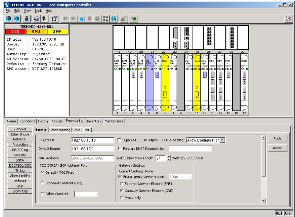
Figure 19-11 Proxy Server Gateway Settings (ETSI only)
