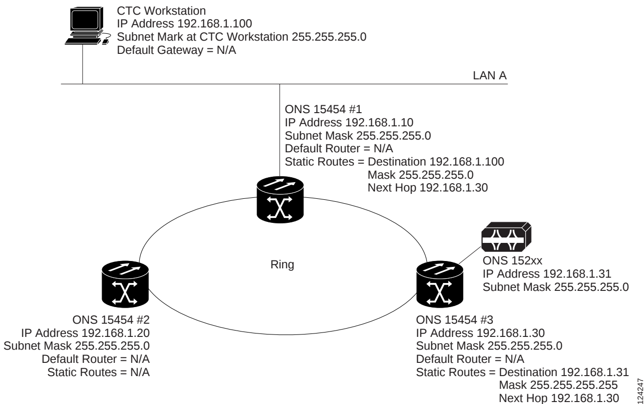
Figure 19-4 Scenario 3: Using Proxy ARP with Static Routing (ANSI and ETSI)
