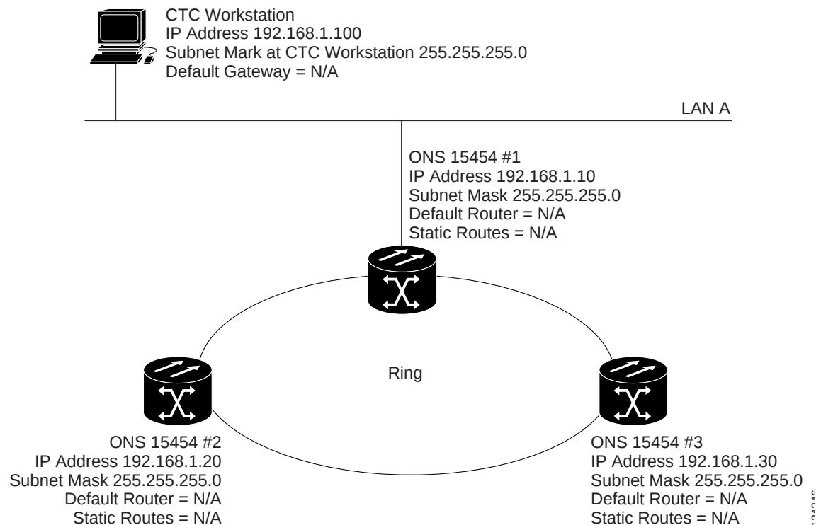
Figure 19-3 Scenario 3: Using Proxy ARP (ANS and ETSII
