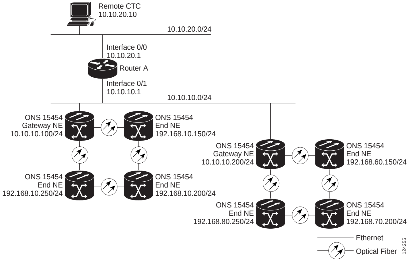
Figure 19-14 Scenario 7: ONS 15454 Proxy Server With ENEs on Multiple Rings (ANSI and ETSI)
