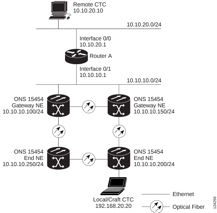
Figure 19-15 Scenario 8: Dual GNEs on the Same Subnet (ANSI and ETSI)
