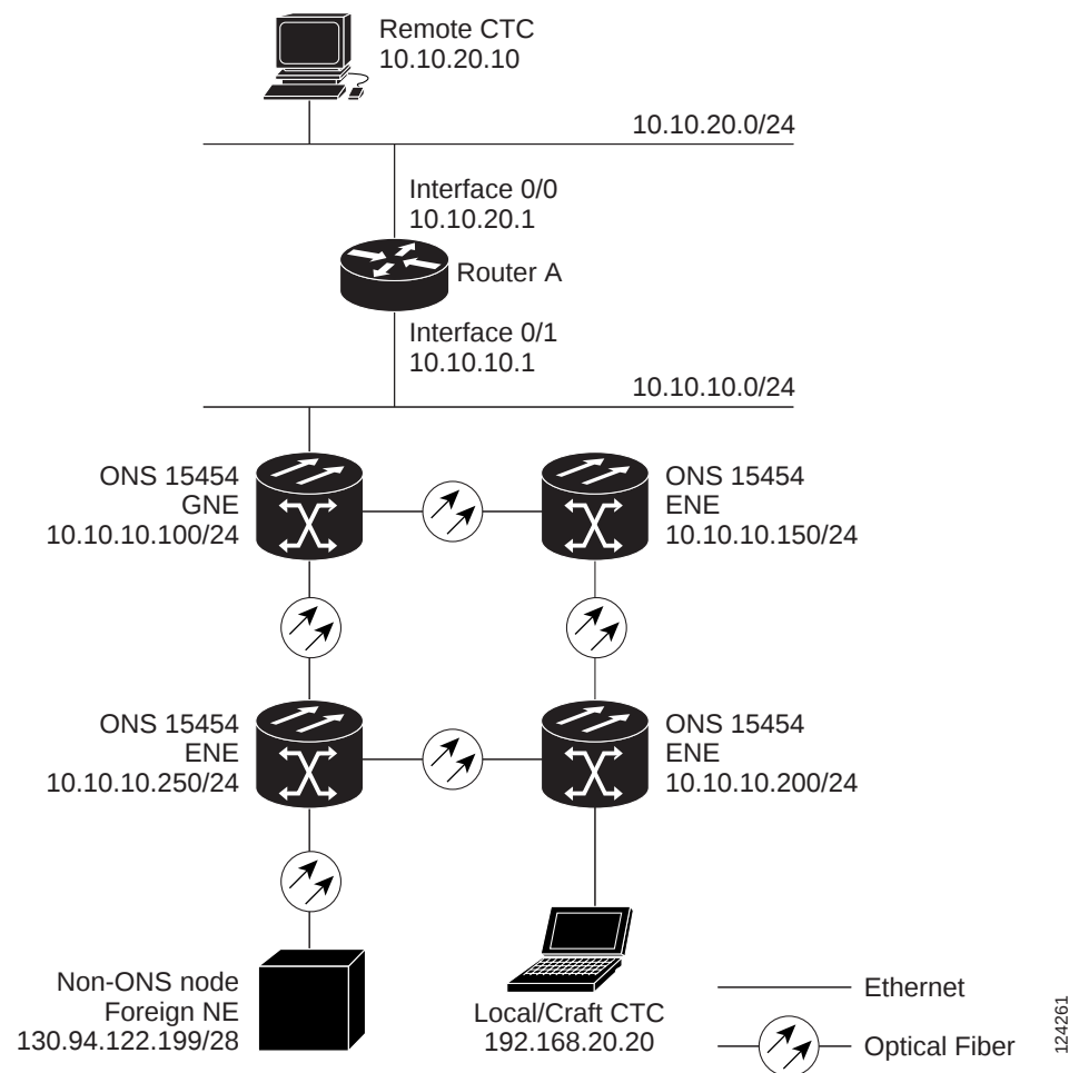
Figure 19-17 Proxy and Firewall Tunnels for Foreign Terminations
