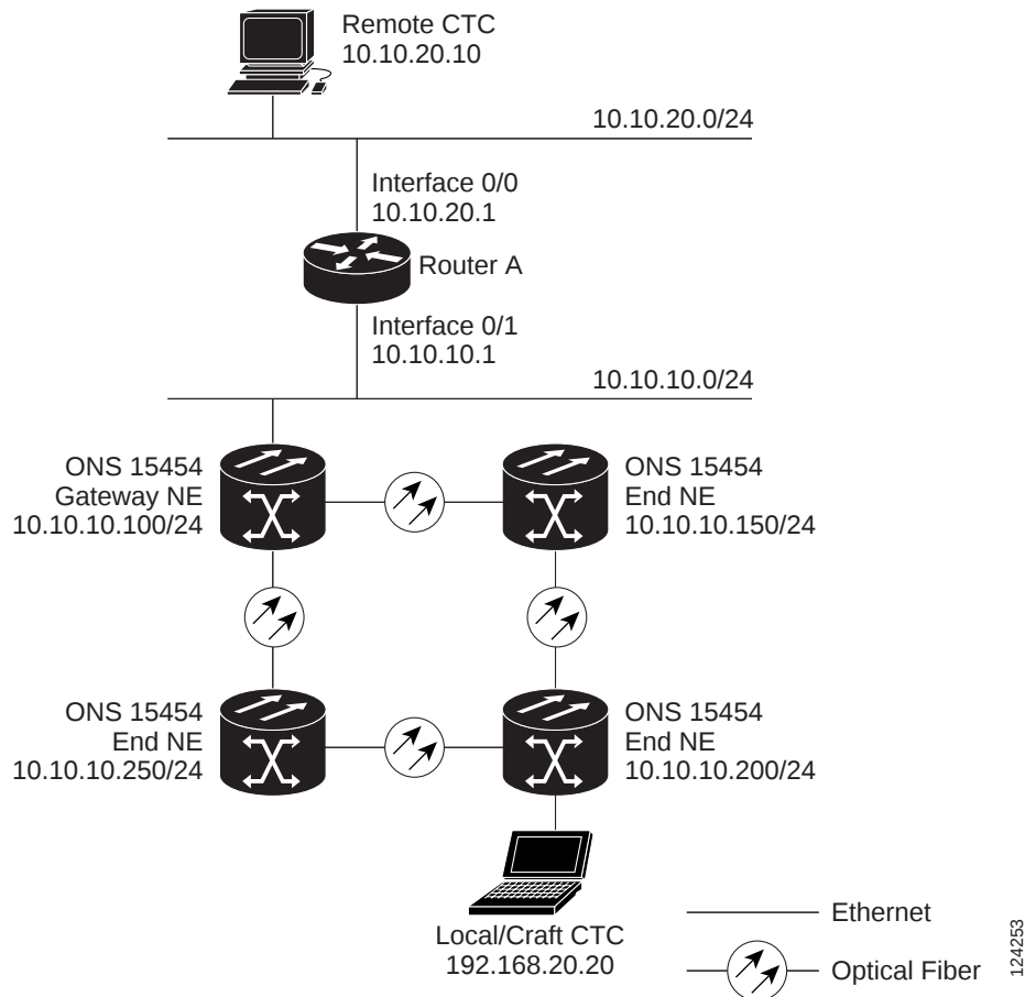
Figure 19-12 ONS 15454 Proxy Server with GNE and ENEs on the Same Subnet (ANSI and ETSI)
