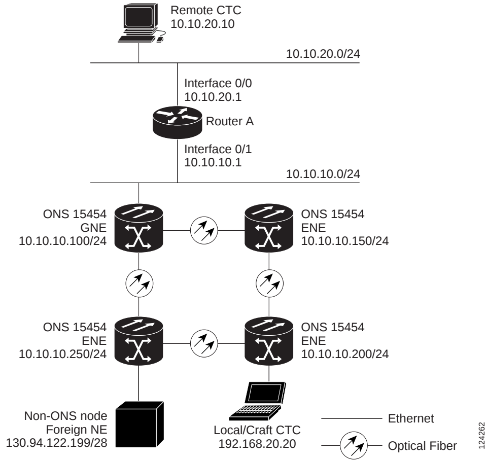
Figure 19-18 Foreign Node Connection to an ENE Ethernet Port
