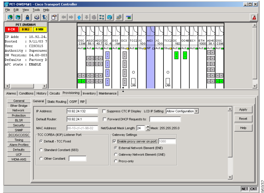
Figure 19-10 Proxy Server Gateway Settings (ANSI only)
