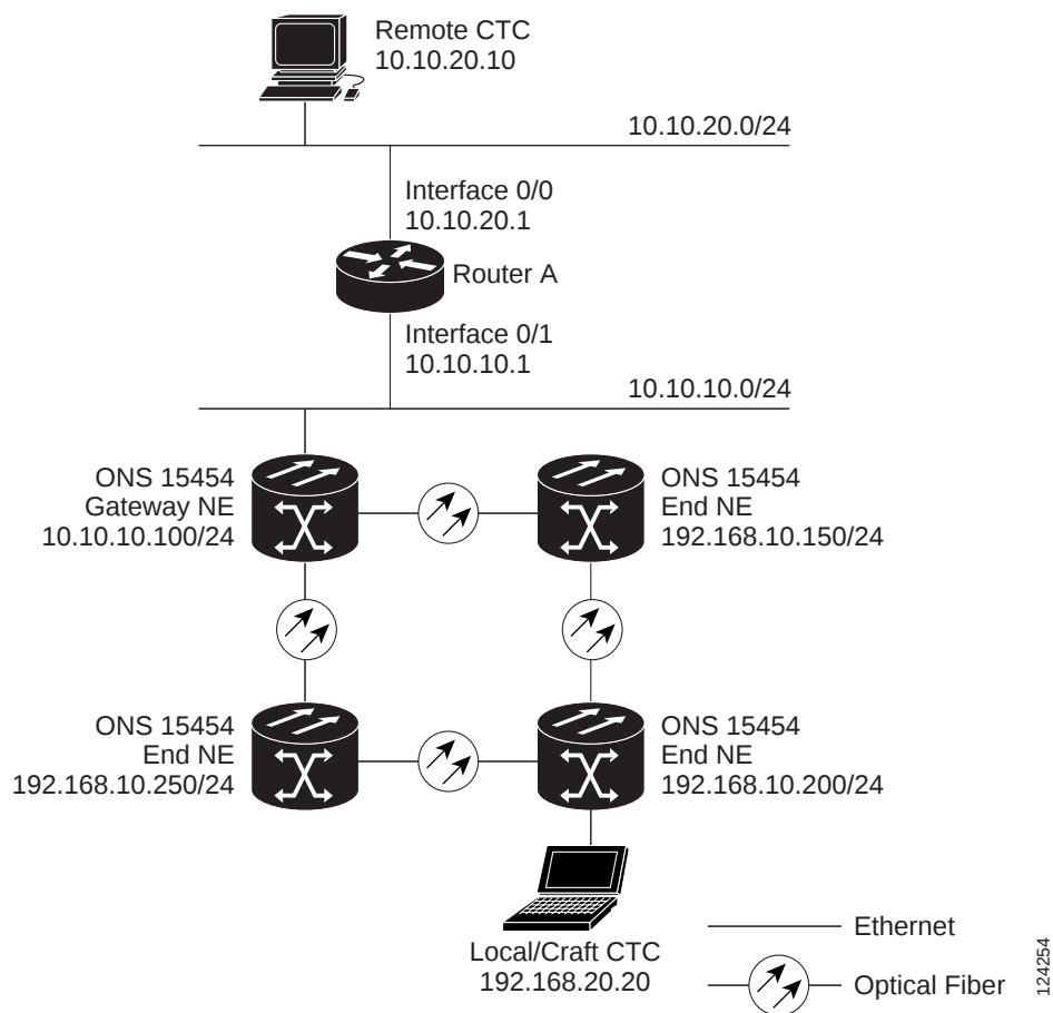
Figure 19-13 Scenario 7: ONS 15454 Proxy Server with GNE and ENEs on Different Subnets (ANSI and ETSI)
