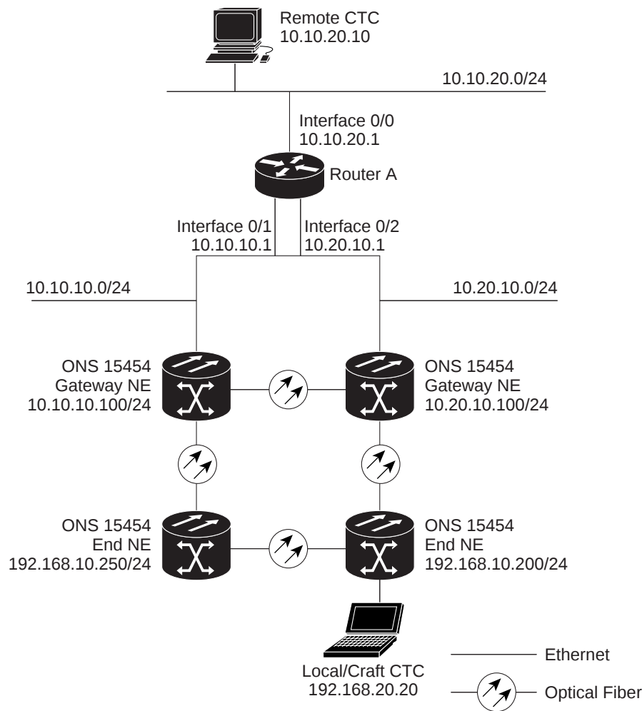
Figure 19-16 Scenario 8: Dual GNEs on Different Subnets (ANSI and ETSI)
