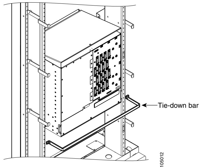
Figure 1-21 Tie-Down Bar
