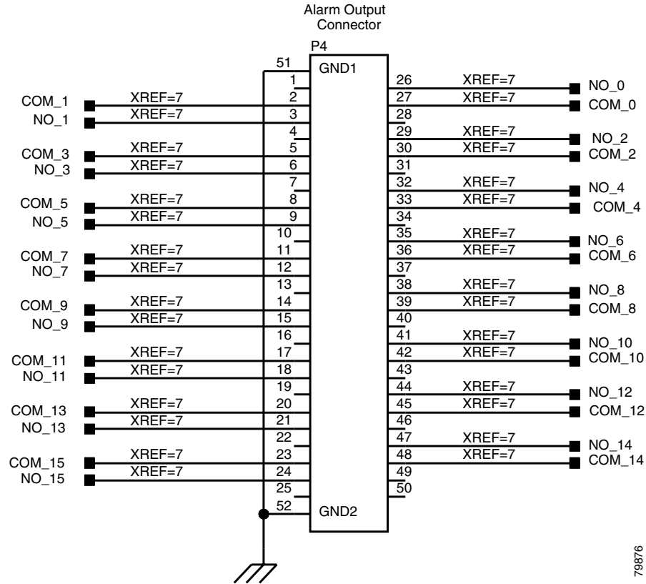
Figure 1-20 Alarm Output Connector
