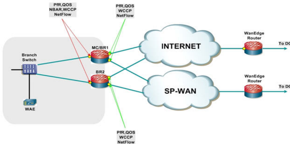
Figure 9-38. Typical Medium Branch Office
