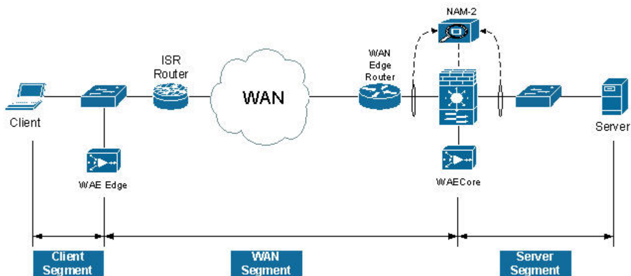
Figure 9-78. NAM-2 Monitoring Segments in the Presence of WAAS
