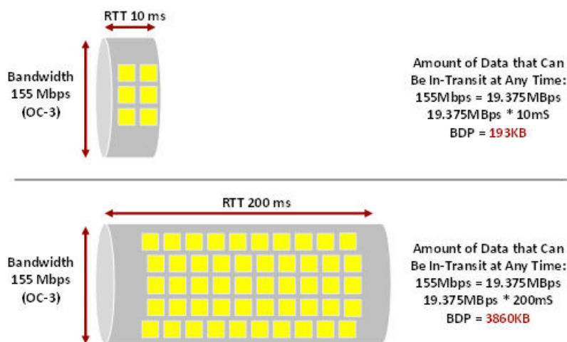
Figure 6-5. Comparing BDPs
