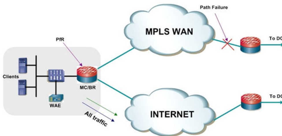
Figure 9-16. SOHO Branch Path Failure with PfR Path Optimization
