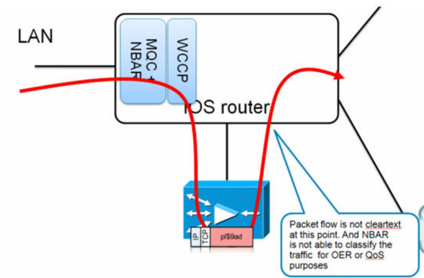
Figure 9-6. NBAR Application Marking with TCP Optimization
