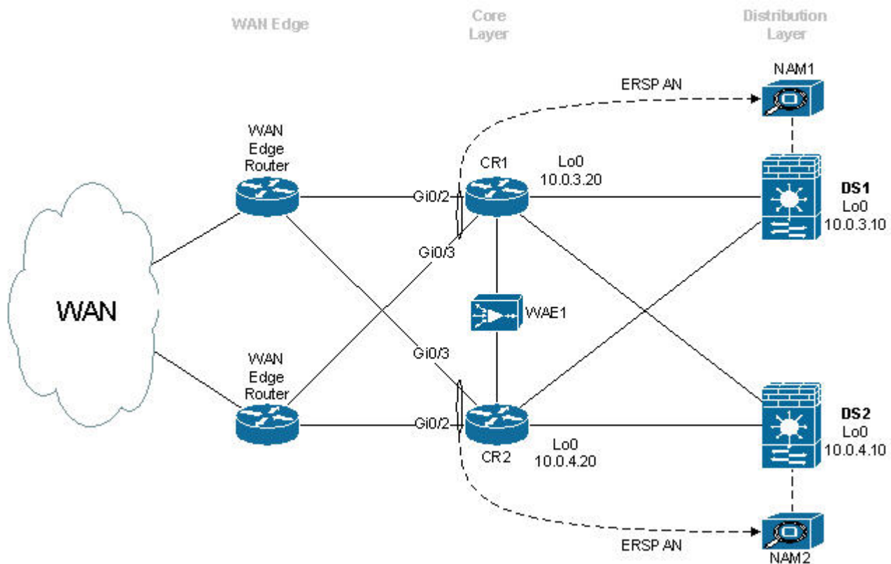
Figure 9-85. ERSPAN Configuration Example
