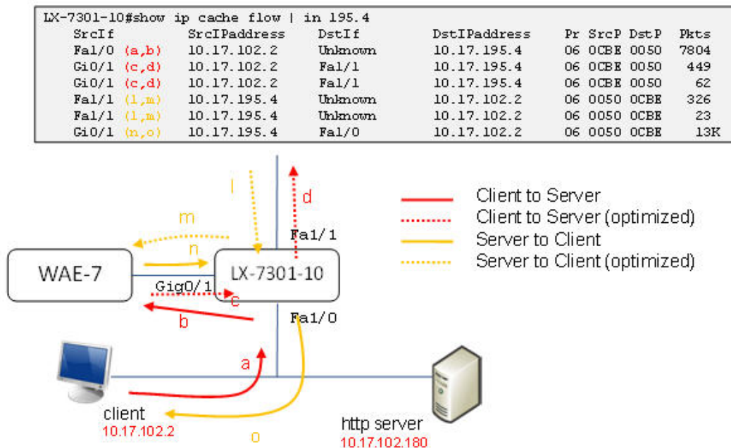
Figure 9-26. NetFlow and WCCP (NetFlow, WCCP, IP return (12.4T))
