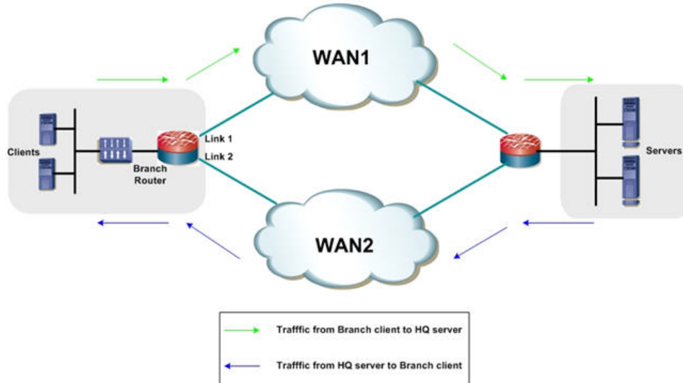
Figure 9-3. Asymmetric Routing
