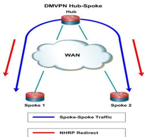
Figure 9-32. DMVPN-NHRP Redirect
