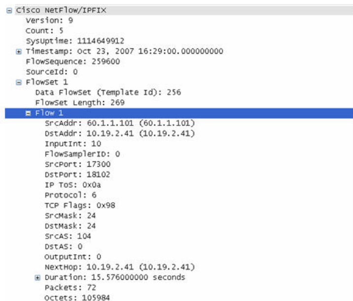
Figure 4-8. NetFlow version 9 Flow Record
