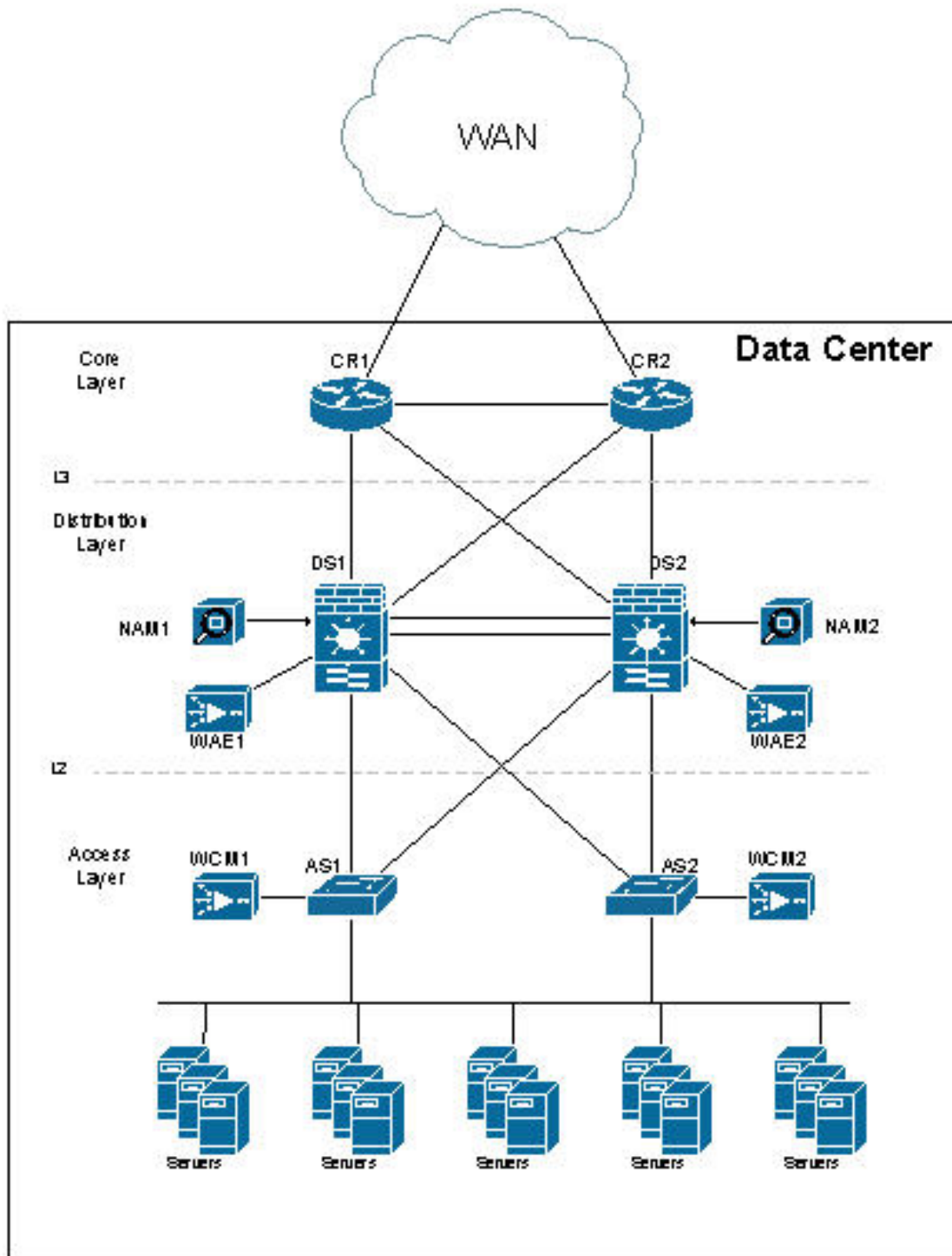
Figure 9-79. Data Center WAAS Deployment Scenario 1
