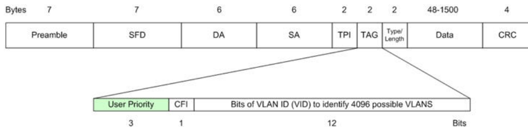
Figure 5-4. Ethernet 802.1Q Frame
