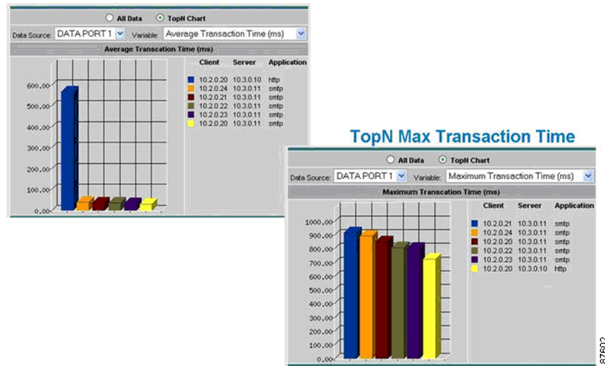
Figure 8-21 Application Response-Time Monitoring
