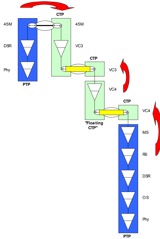
Figure Error! No text of specified style in document.-6. Modeling with Floating CTPs (elevation)
