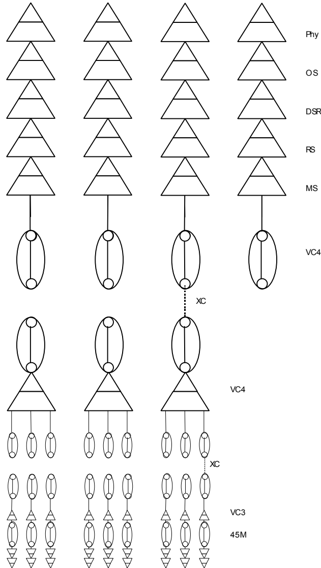
Figure Error! No text of specified style in document.-5. G.805 modeling example ("plan" view)
