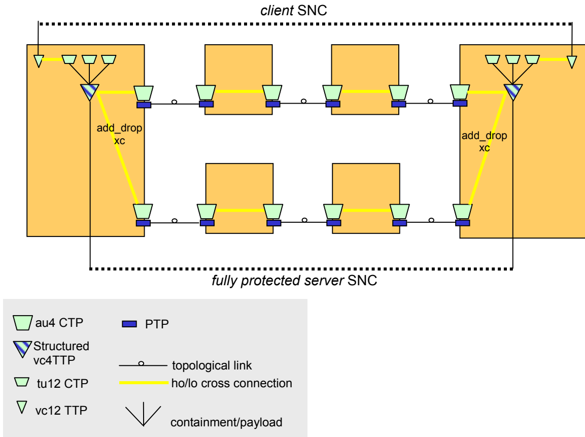
Figure Error! No text of specified style in document.-10. Protected Trail using FTPs
