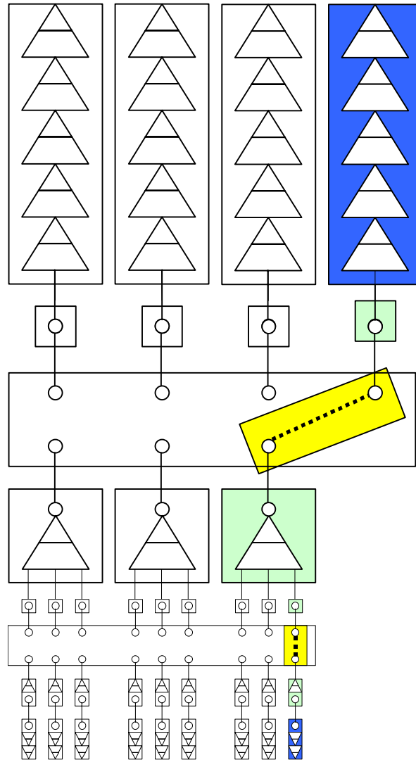
Figure Error! No text of specified style in document.-8. Modeling with Floating CTPs (plan): Example of cross-connects
