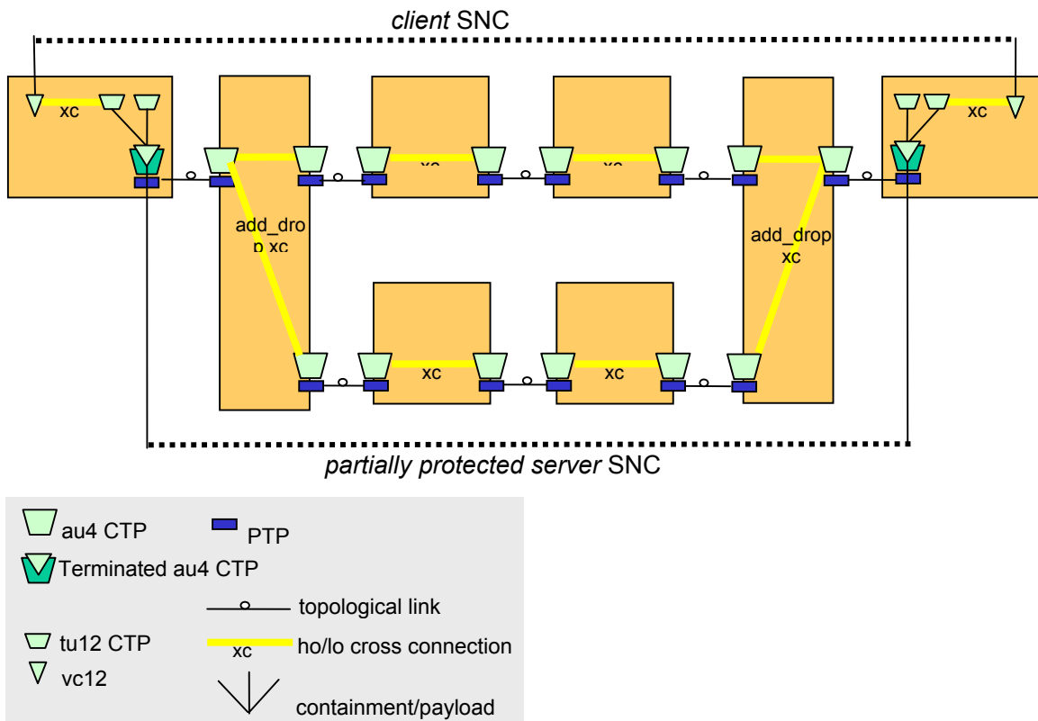
Figure Error! No text of specified style in document.-9. Partial SNC Protection without FTPs
