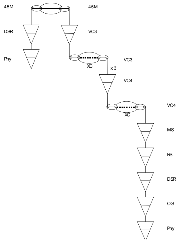
Figure Error! No text of specified style in document.-4. G. 805 modeling example ("elevation" view)
