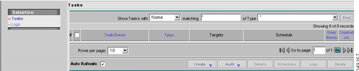
Figure 7-9 Tasks
