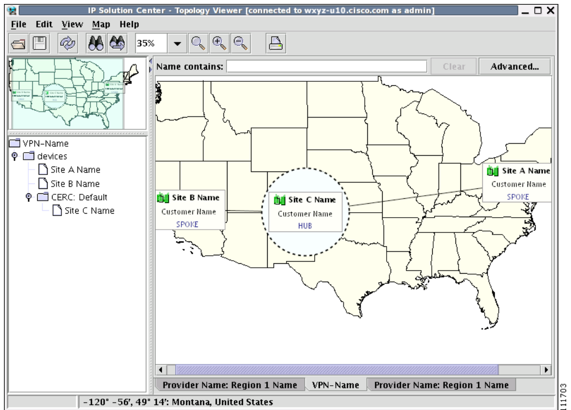
Figure 3-68 Map Layers
