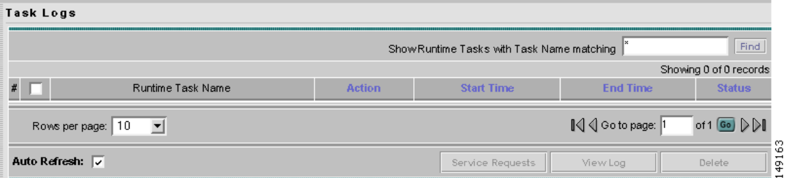
Figure 7-10 Task Logs
