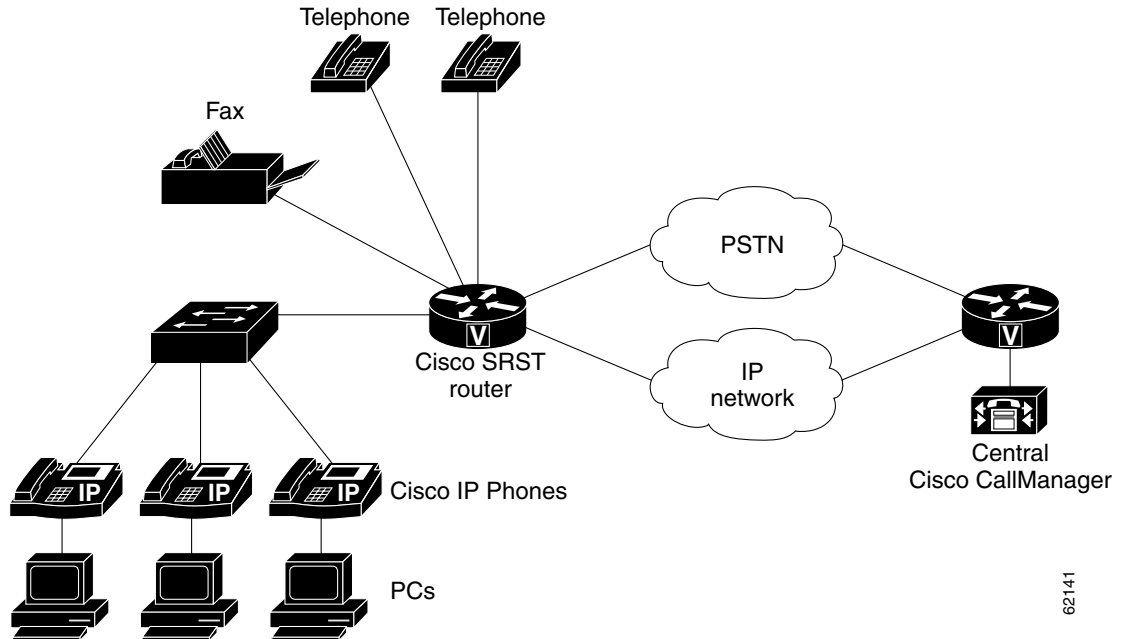
Figure 18-1 Branch Office Cisco IP Phones Connected to a Remote Central Cisco CallManager
