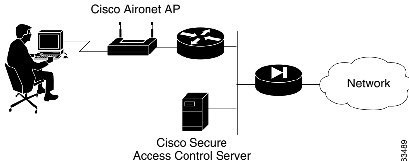
Figure 2-4 Simple WLAN
