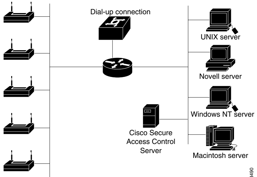
Figure 2-5 Campus WLAN
