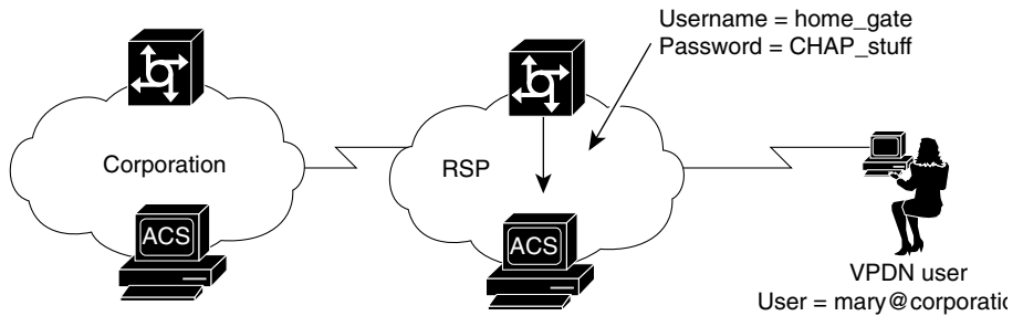
Figure D-7 NAS Authenticates Tunnel with ACS
