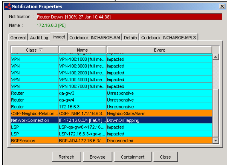
Figure 8: Notification Properties Dialog Box Showing a Router Down Problem
