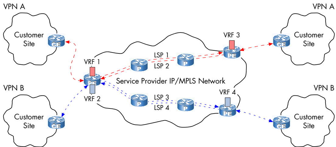
Figure 15: MPLS-Capable IP Network and MPLS VPNs
