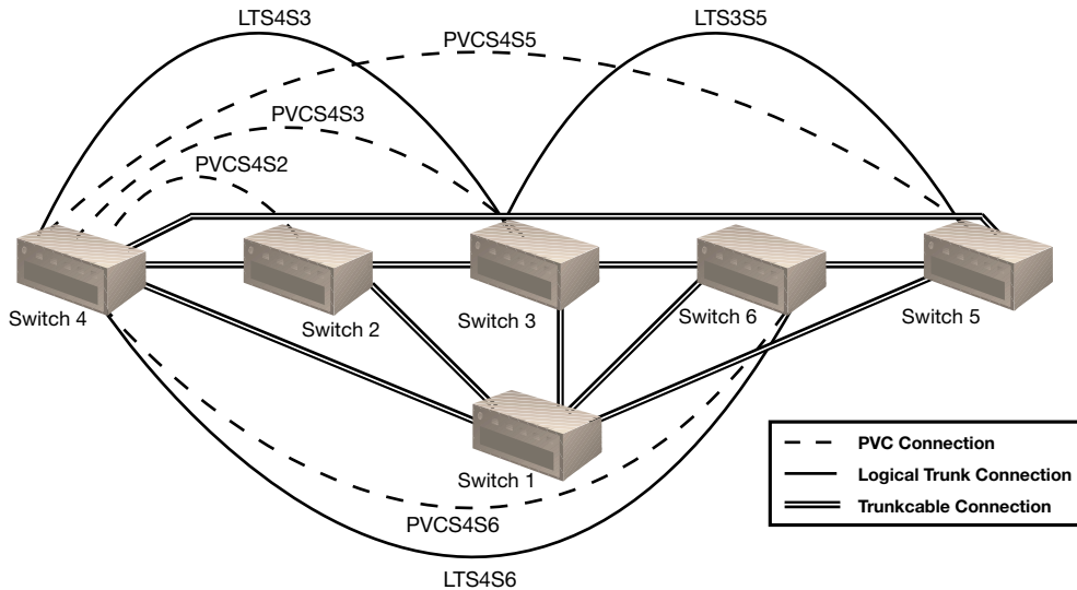
Figure 5: Physical and Logical Connectivity
