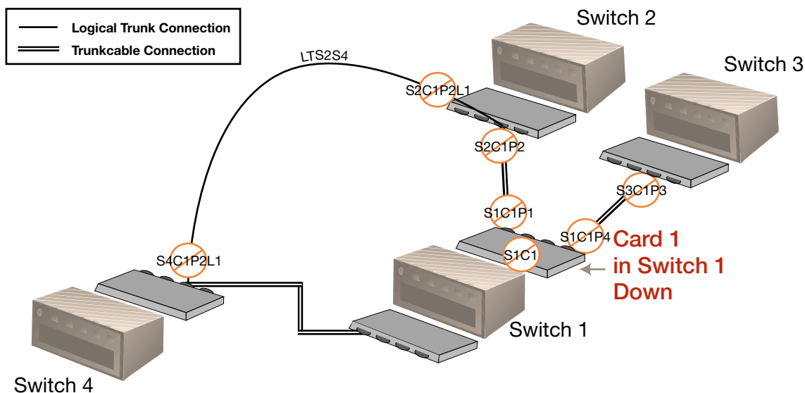
Figure 10: Card Down Scenario
