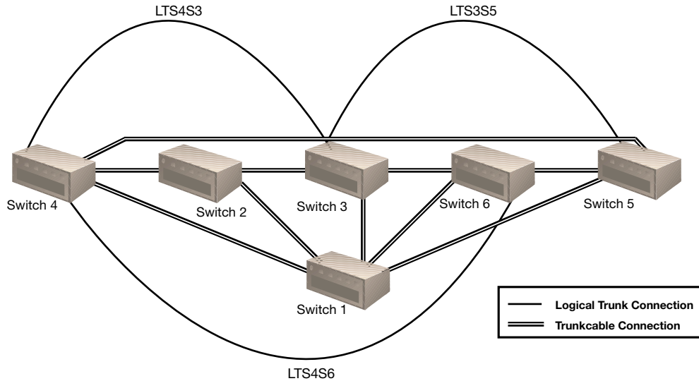
Figure 4: Logical Trunk Connectivity
