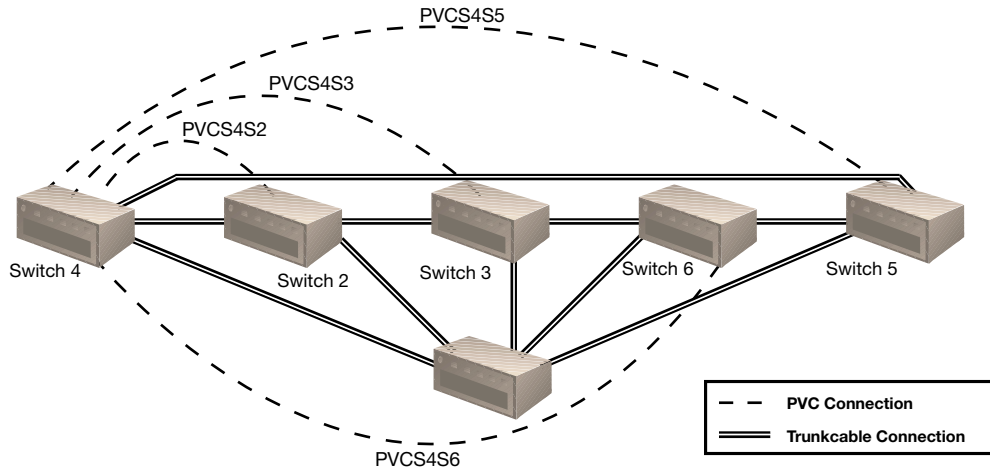
Figure 3: Permanent Virtual Circuit (PVC) Connectivity
