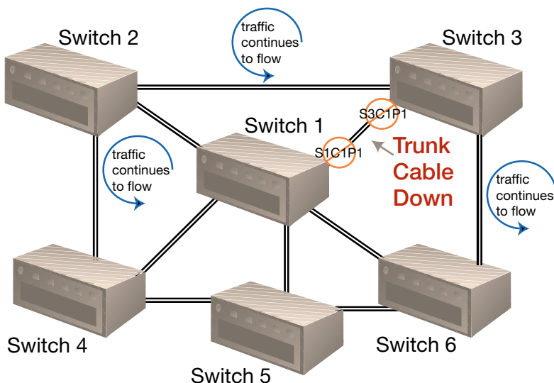
Figure 7: Trunk Cable Down
