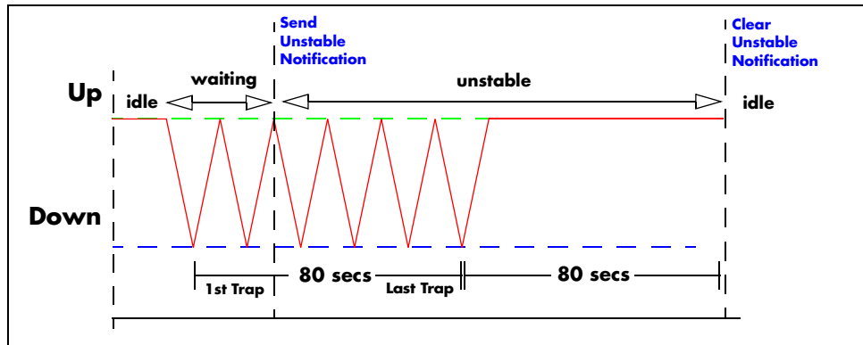
Figure 11: Unstable System/Network Adapter Diagnosis
