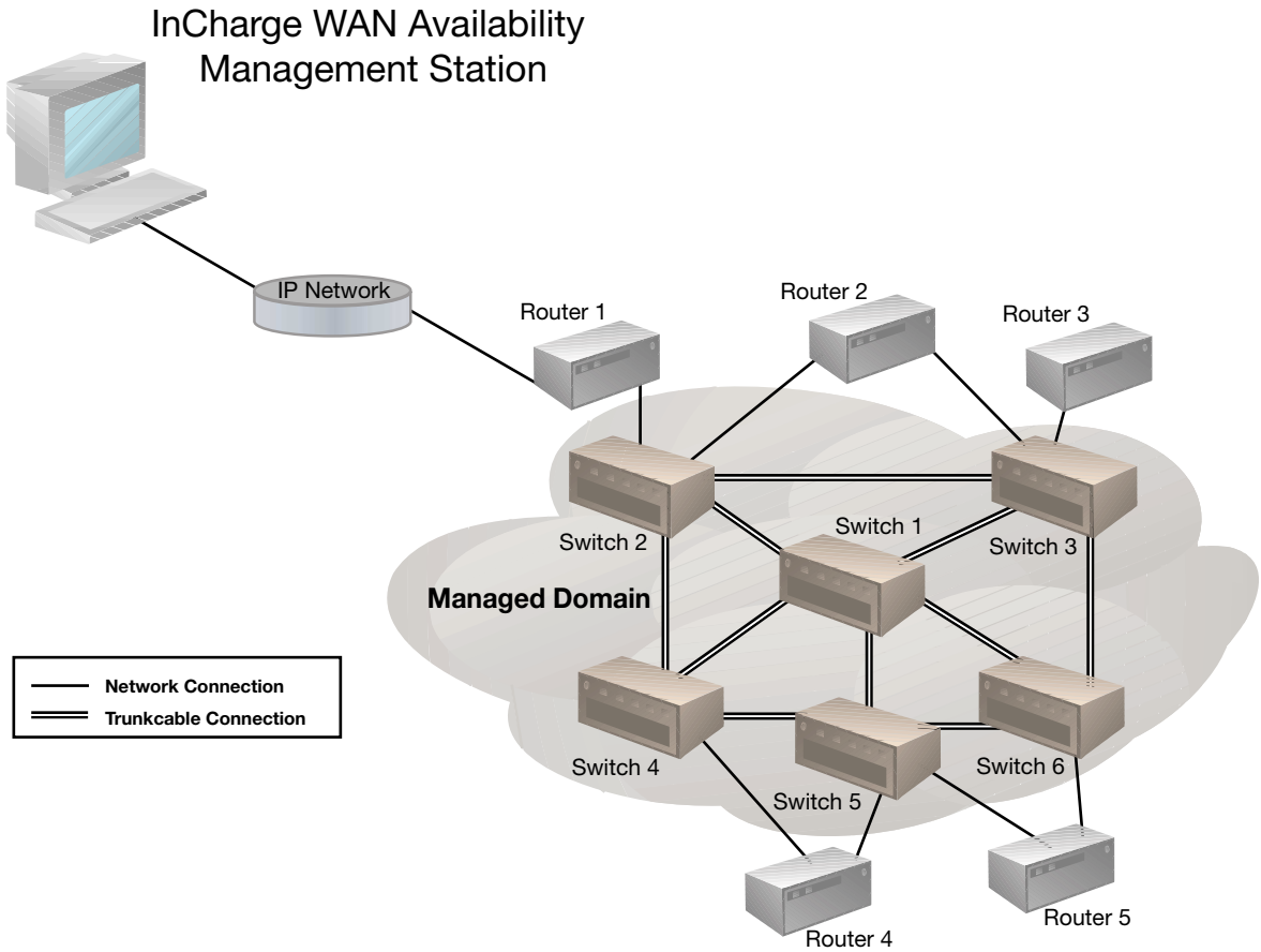
Figure 1: Typical WAN Architecture
