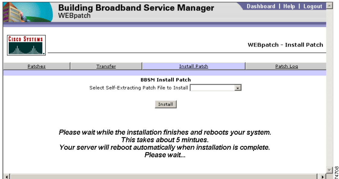
Figure 3 WEBpatch Install Patch Web Page
