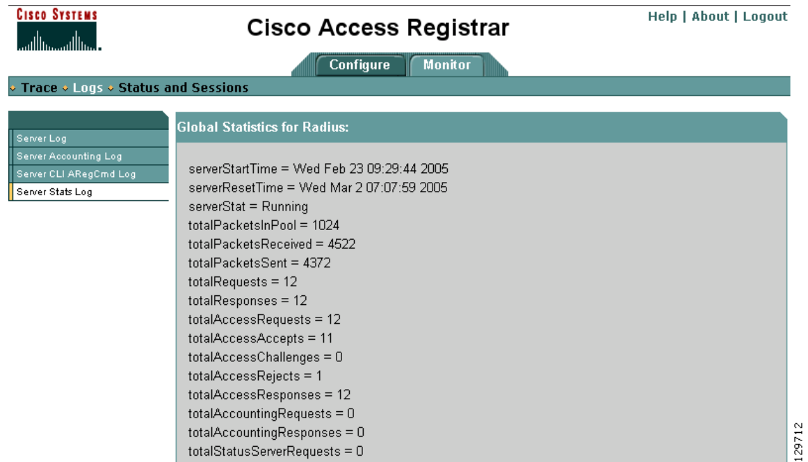
Figure 3-25 Server Statistics Log
