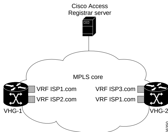
Figure 11-1 MPLS Core
