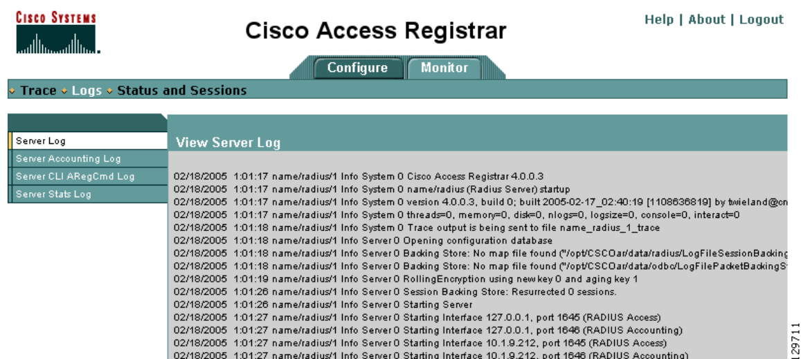
Figure 3-22 Server Log Page
