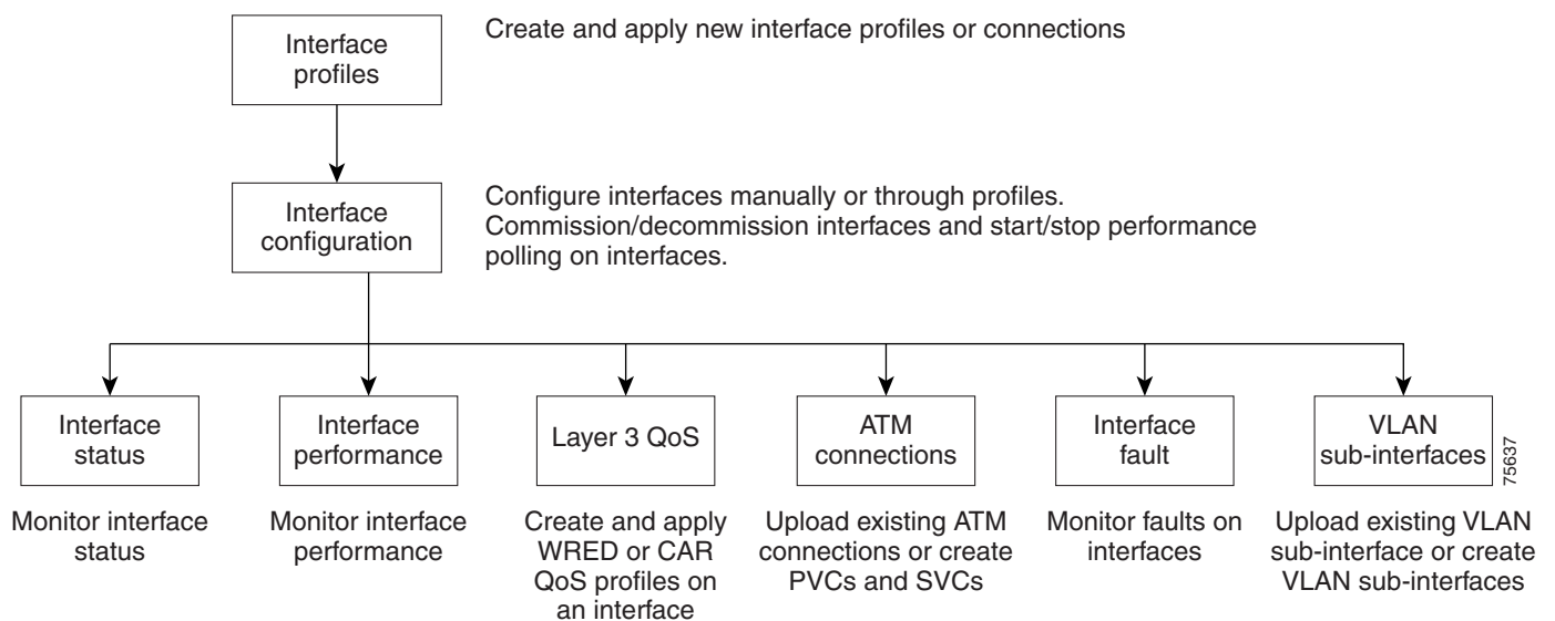
Figure 6-1 Managing Interfaces
