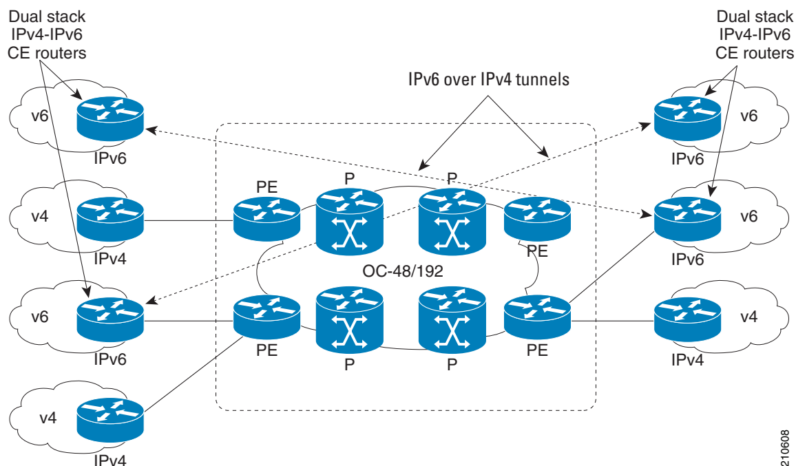
Figure 22 IPv6 Using Tunnels on the CE Routers
