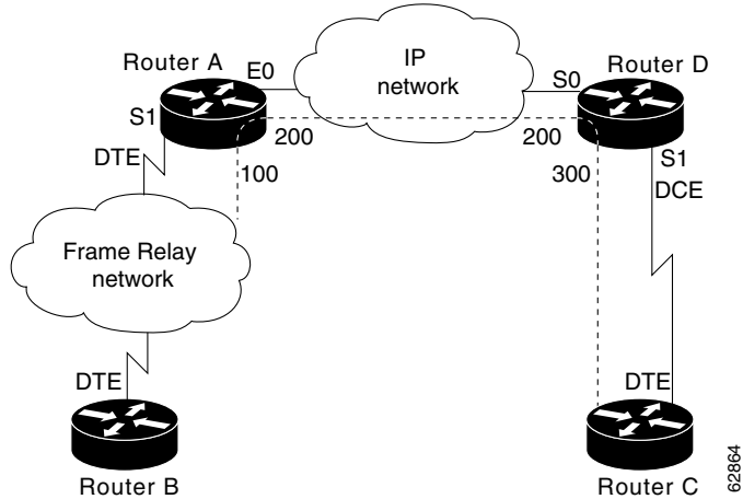
Figure 13 Frame Relay Switch over IP Tunnel
