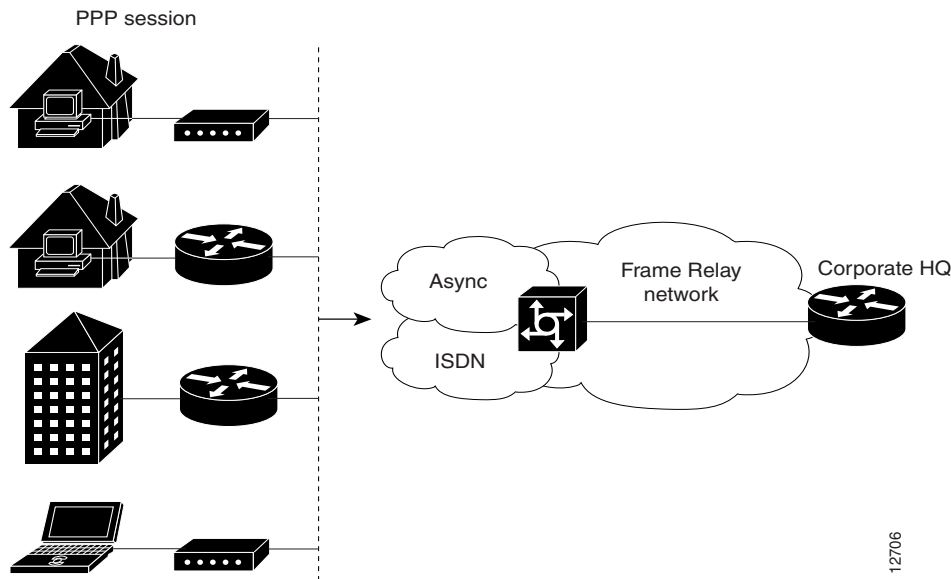
Figure 8 PPP over Frame Relay Scenario
