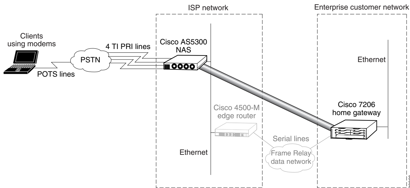
Figure 15 Access VPN Topology Using Local AAA
