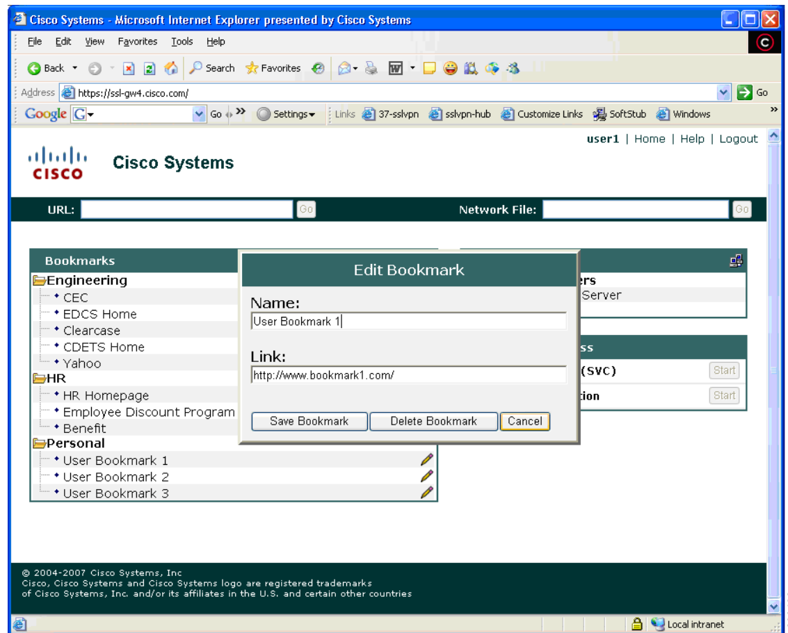
Figure 18 Edit Bookmark
