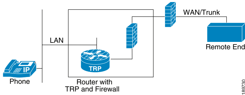
Figure 1 Architecture for Cisco IOS Firewall in a TRP Network Solution
