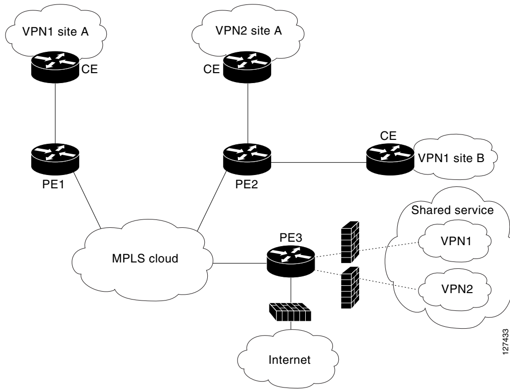
Figure 38 Hub-and-Spoke Network
