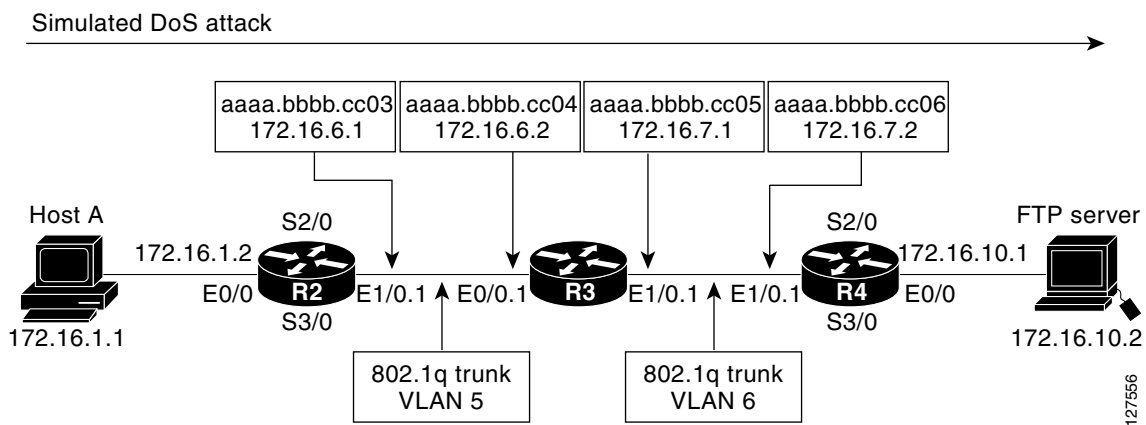
Figure 7 Test Network
