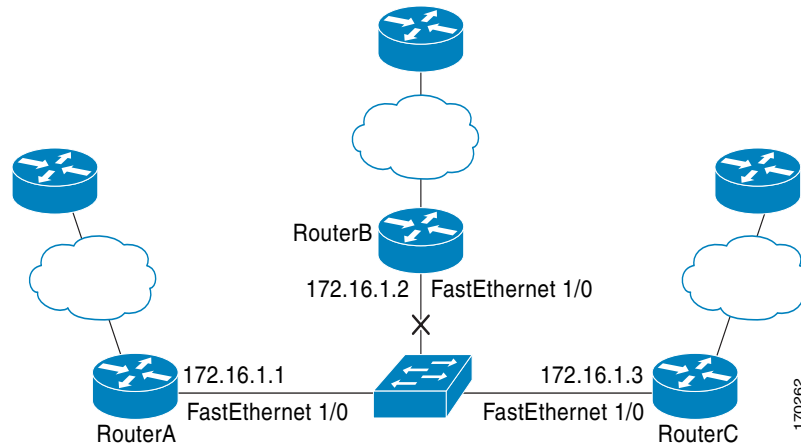
Figure 4 Fast Ethernet interface 0/1 Failure
